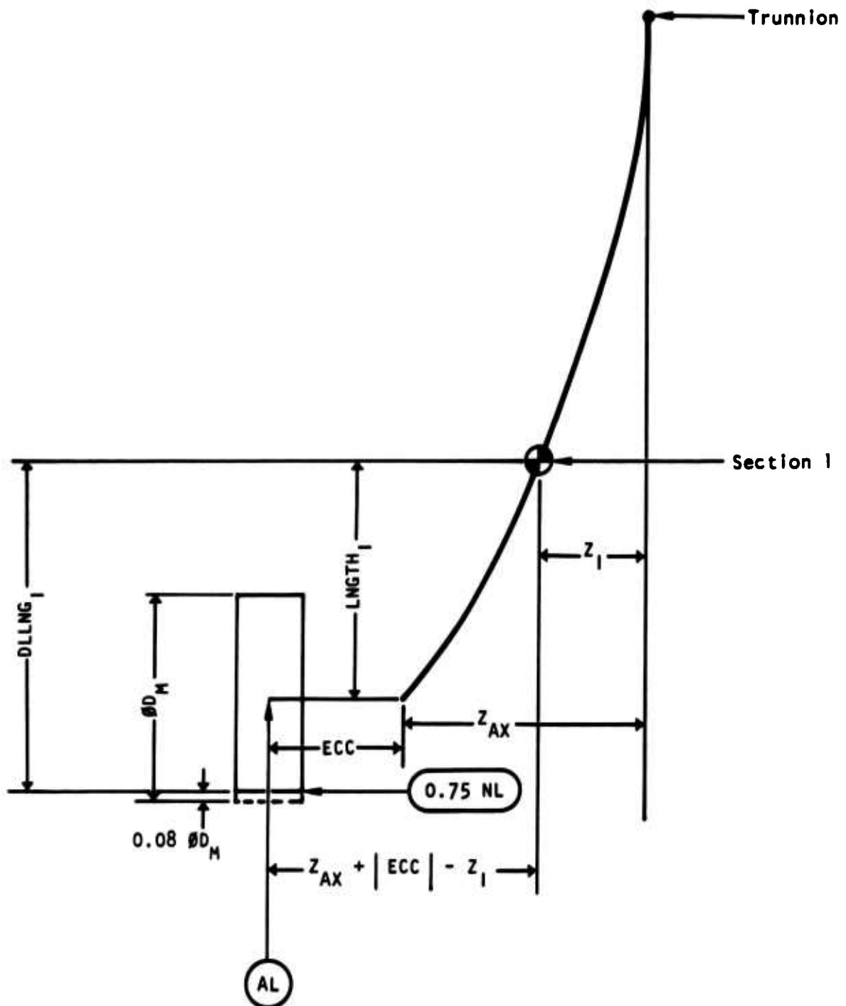
Figure 44. Lateral bending moment for drift landing when the eccentricity is negative and greater than one-tenth the length to the ground.
