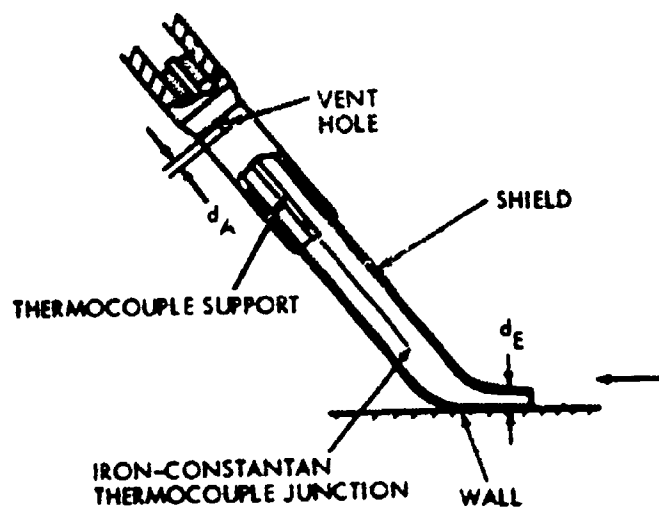
FIG. 2 SHIELDED THERMOCOUPLE PROBE (11)
