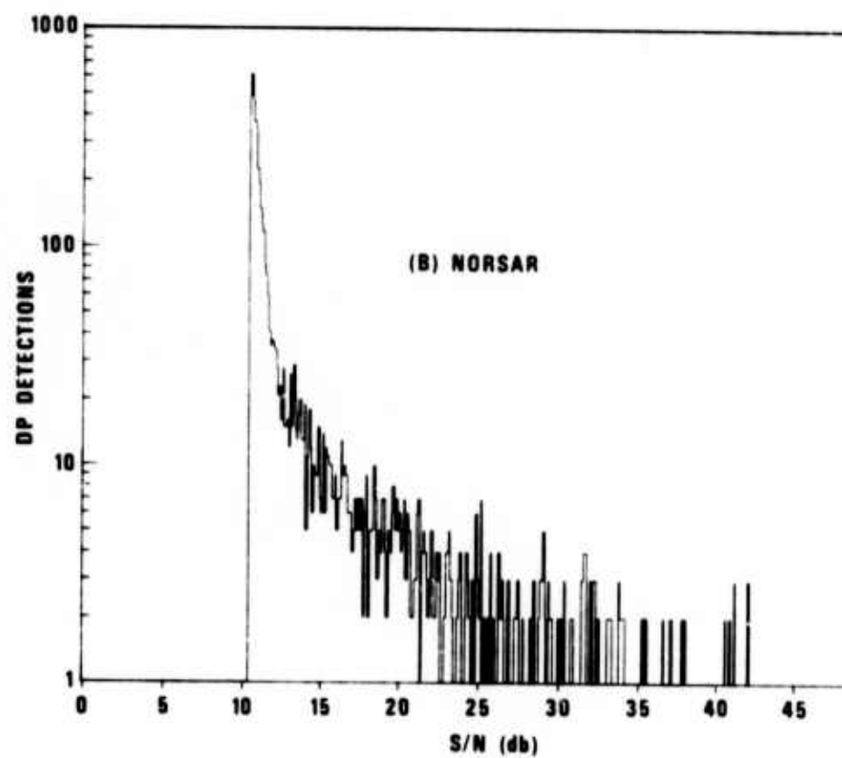
Figure 7. LASA and NORSAR discrete DP recurrence curves.
