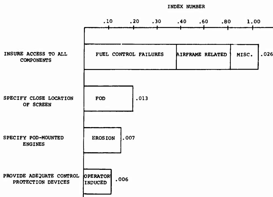
Figure 38. Remedial Action Subgroups for Additional Control of Engine/Airframe Interface for Composite Baseline.
