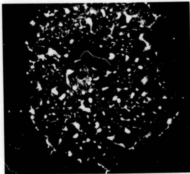
Fig. 4-9(b) SEM micrograph of "multiple" SQBD on (100) n-type substrate with Al(-). d_o = 2500\text{\AA} , V_b \sim 185\text{ V} , T = 100\text{ K} x2,000
