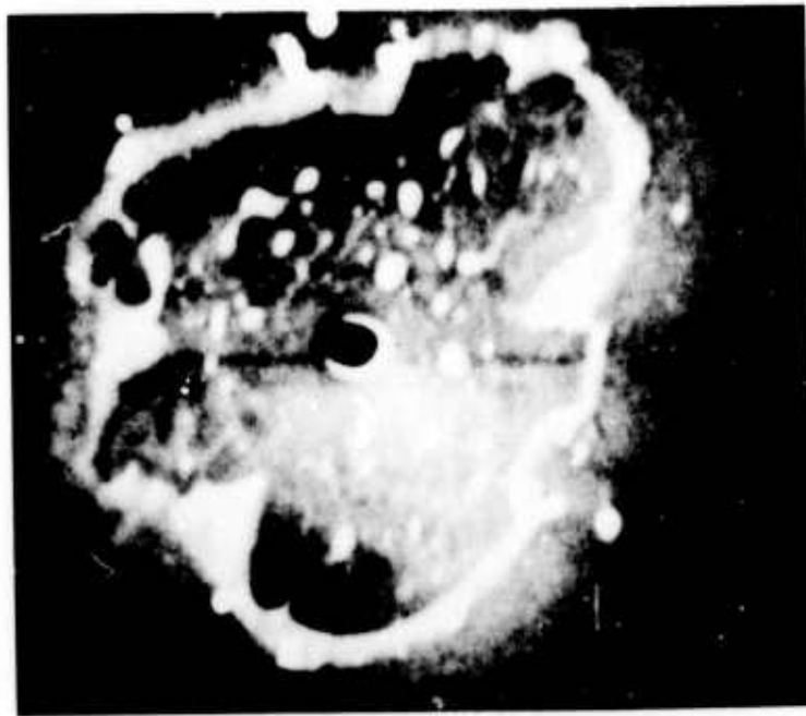
Fig. 4-9(a) SEM micrograph of single SQBD on (100) n-type substrate with Al(-). d_o = 2500\text{\AA} . V_b \sim 185\text{V} , T = 300\text{ K} x5,000
