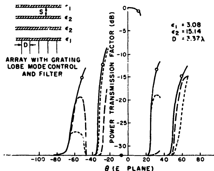
Figure 12. Limited-Scan Array Grating Lobe Amplitude Locus [ \cdots — odd-mode scanning no filter; ---- odd-mode scanning with four-layer Chebyshev filter ( S=0.5\lambda ); - - - odd-mode scanning with four-layer Chebyshev filter ( S=\lambda )]
