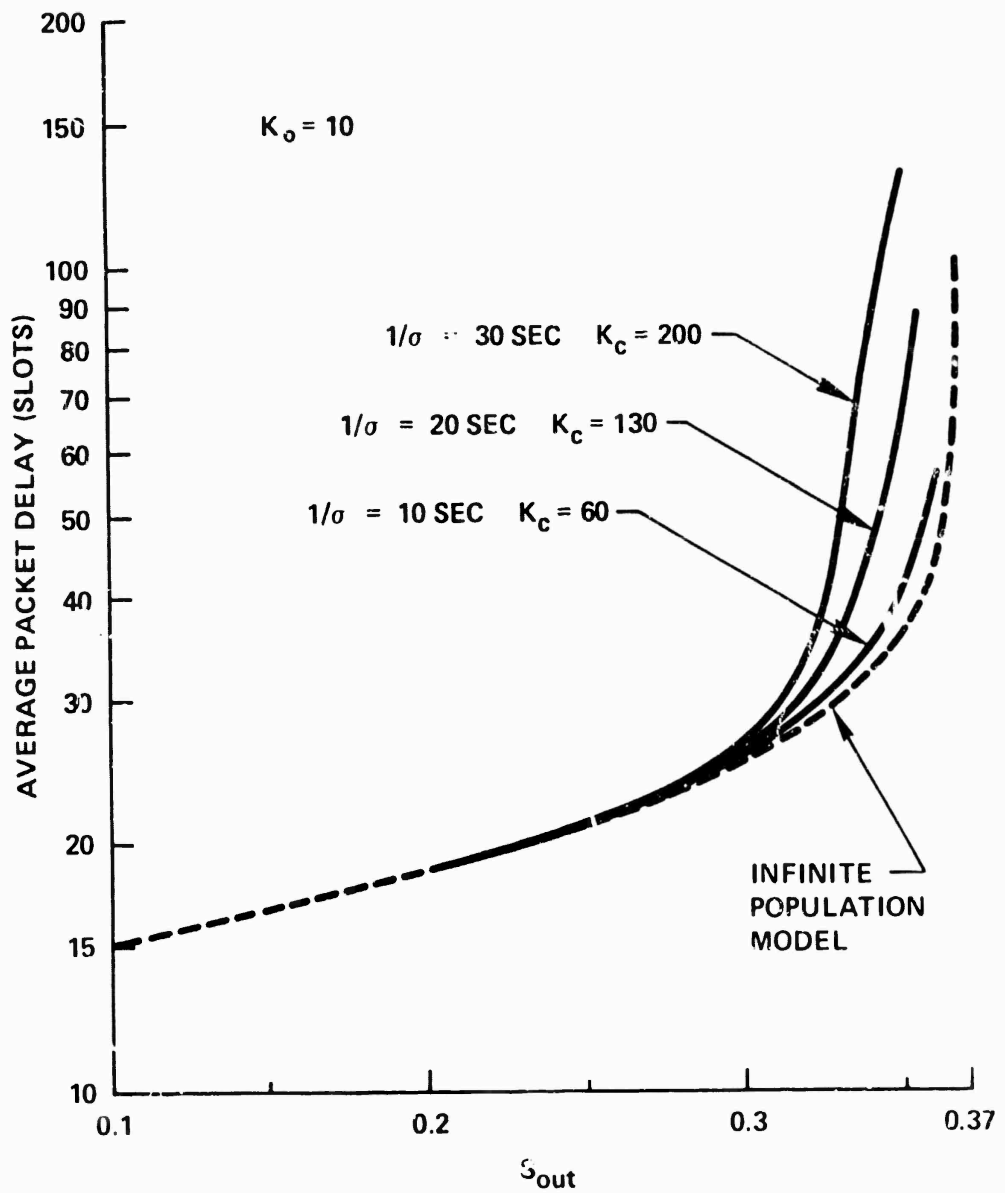
Figure 6-20. RCP Optimum Throughput-Delay Tradeoffs at Fixed \sigma .
