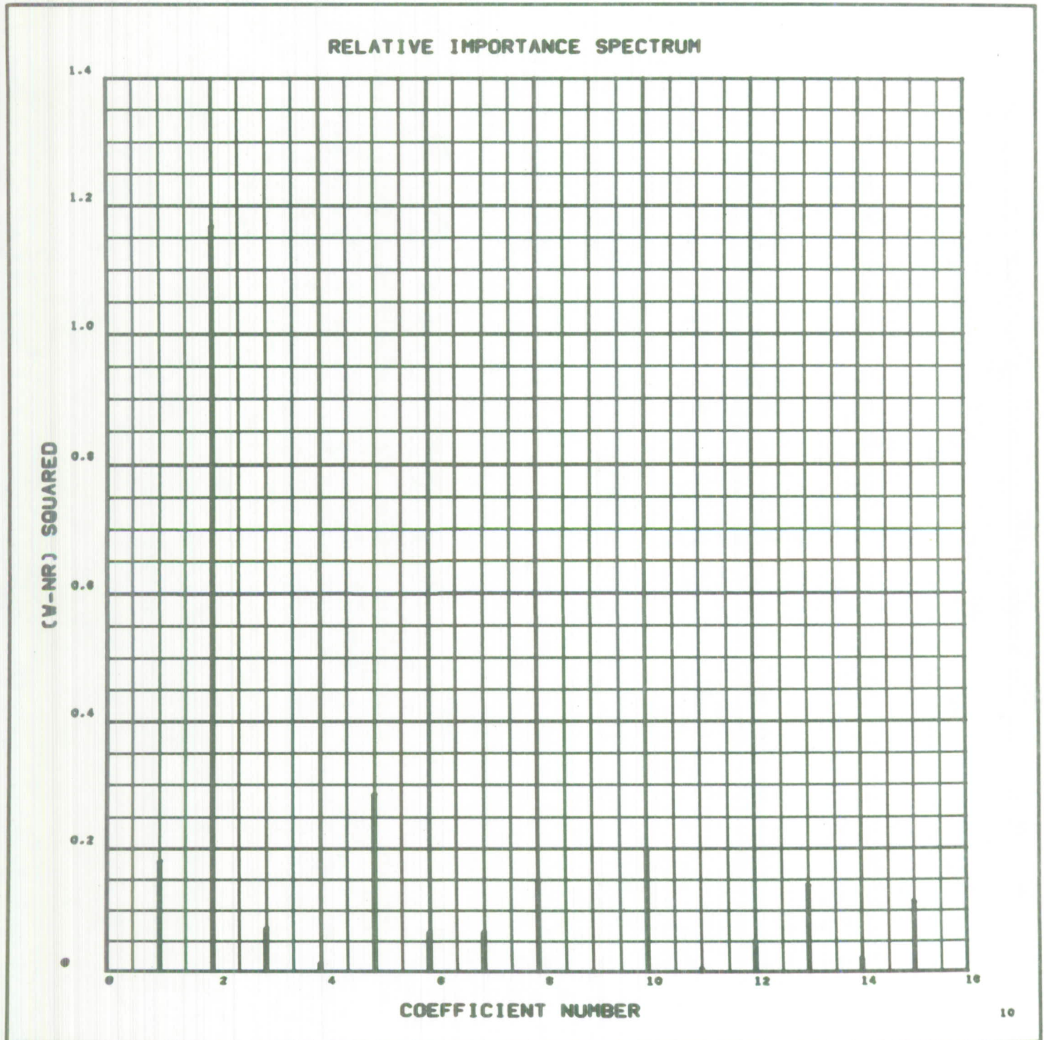
FIGURE 4.33 - RELATIVE IMPORTANCE OF EACH OPTIMAL COORDINATE TO MINIMUM VARIATION RATIO CLASSIFICATION DIRECTION DEVELOPED ON LOW VARIATION BASE
