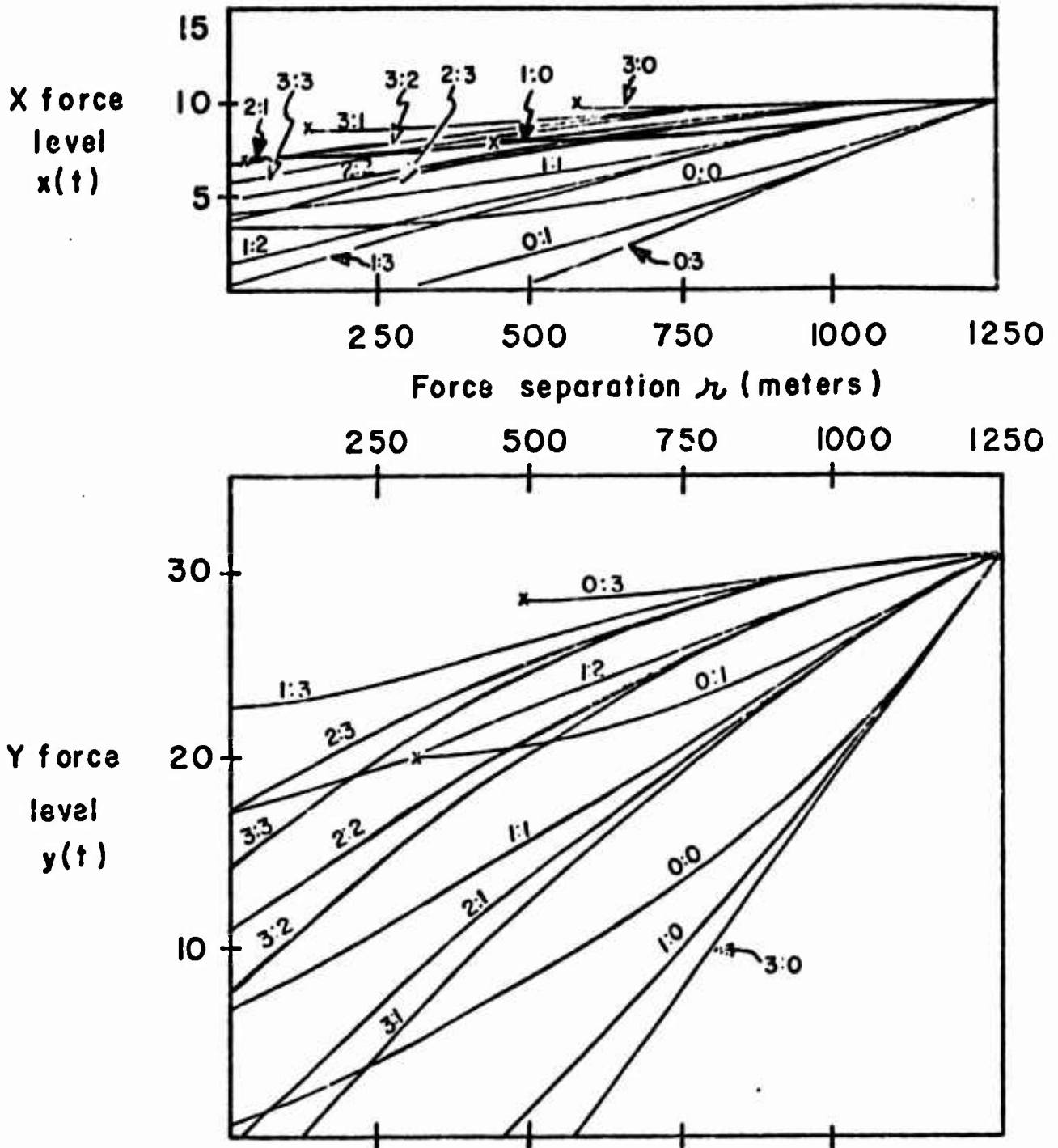
Figure 3. Force-level trajectories of X and Y forces for various combinations of the exponents m and n in the power attrition-rate coefficients for R_0 = 1250 meters, R_\alpha = R_\beta = 2000 meters, \alpha_0 = 0.06 X casualties/(minutes \cdot Y unit), \beta_0 = 0.6 Y casualties/(minutes \cdot X unit), v = 5 mph, x_0 = 10 , and y_0 = 30 . The exponent combinations are denoted as m:n in the figure, and the symbol x denotes the end of a force-level trajectory due to the annihilation of the enemy force.
