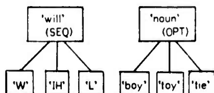
Figure 2. Examples of SEQUENCE and OPTION Relationships.
