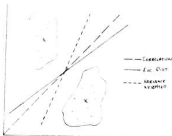
Figure 4 -- Decision Boundaries
