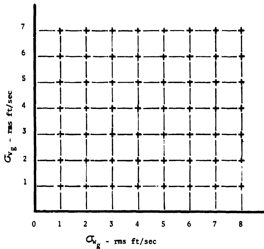
Figure 12 - COMBINED VERTICAL AND LATERAL GUST ENVELOPE FOR A DOUBLE SYSTEM
