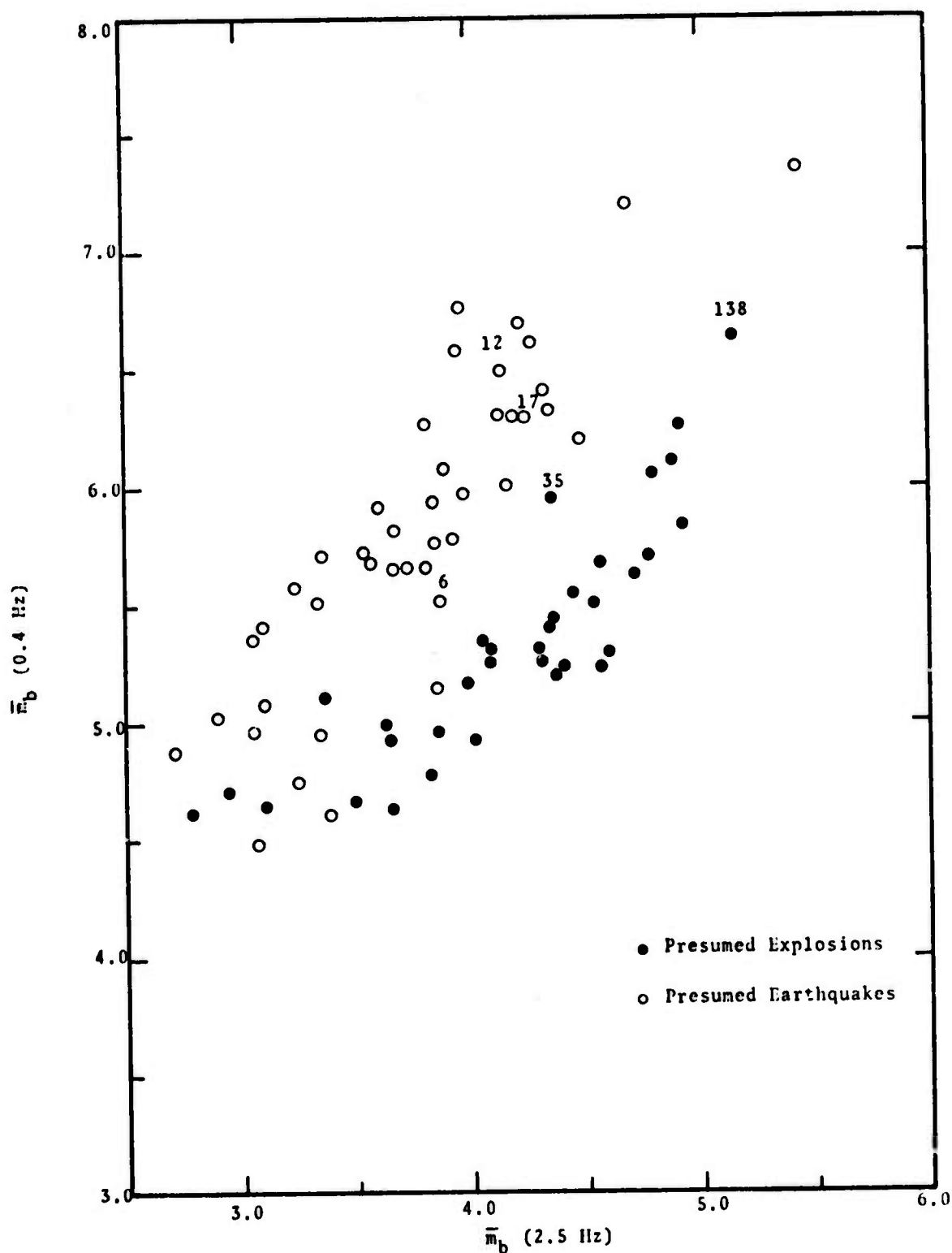
Figure 4.2. Spectral magnitude estimates at 0.4 Hz and 2.5 Hz for the same population of events plotted in Fig. 4.1.
