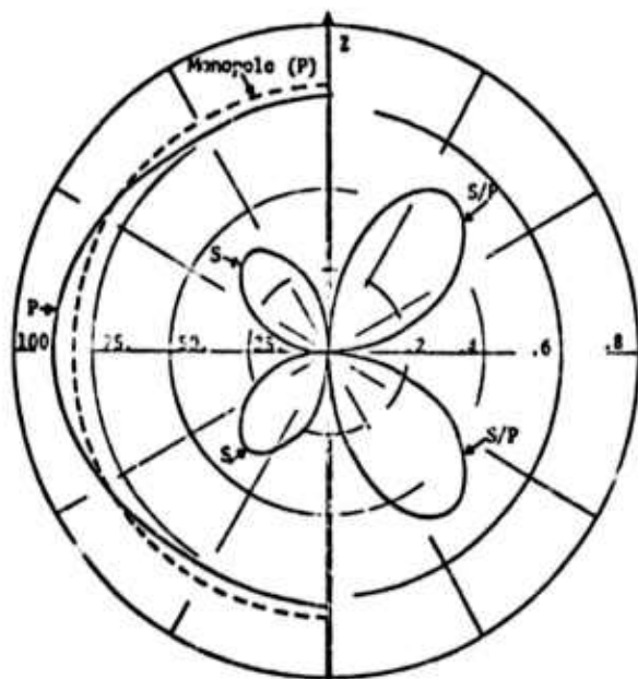
(a) 1 Second radiation pattern.
