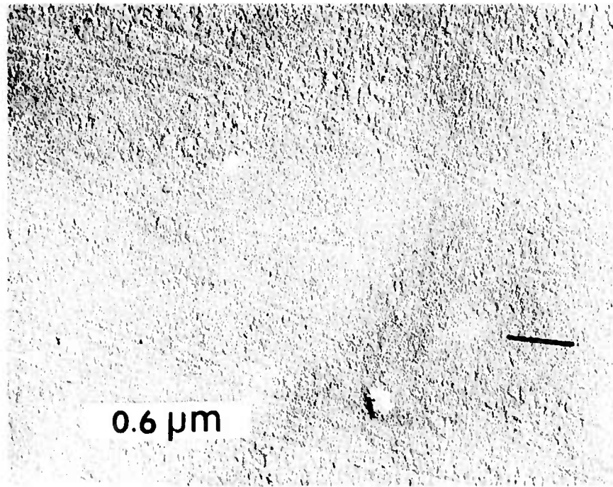
Figure I-10. ED-2 bowl-feed - rouge polished - long polishing time
