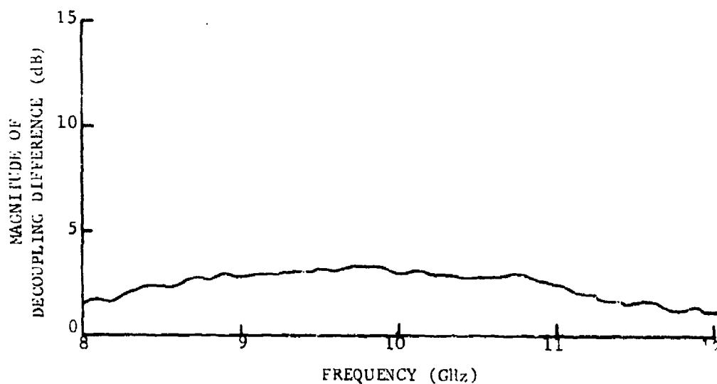
Figure 101. Magnitude of the decoupling difference for the measured data presented in Figure 100.
