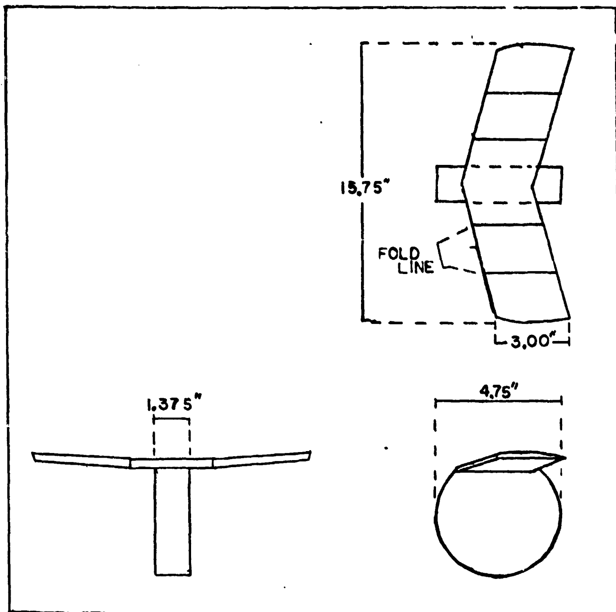
Fig. 1. Wing-Body Configuration
