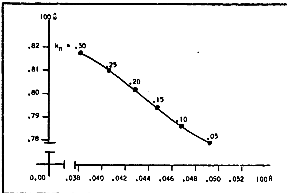
Fig. 11 Root Locus for Wing-Body-Tail for Dutch Roll I
