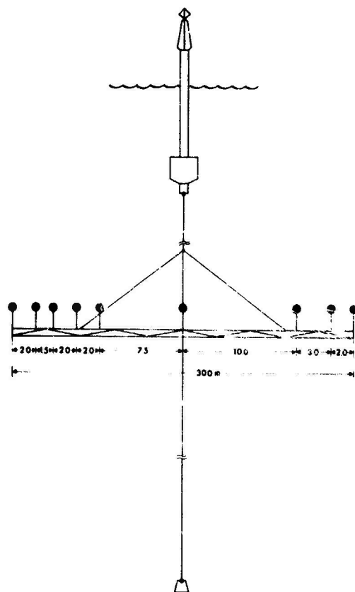
FIG. 2 ARRAY CONFIGURATION
