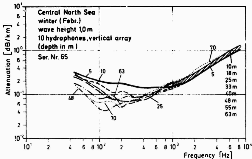
FIG. 17 ATTENUATION FOR DIFFERENT RECEIVER DEPTHS, WINTER CONDITION
