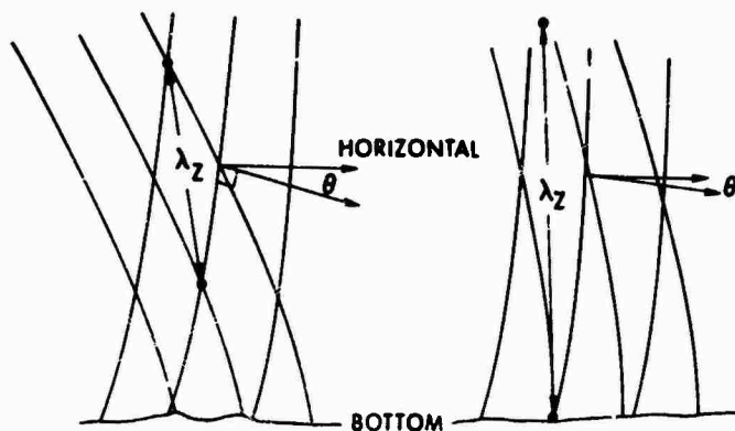
IDEALIZATION OF MODE FORMATION
