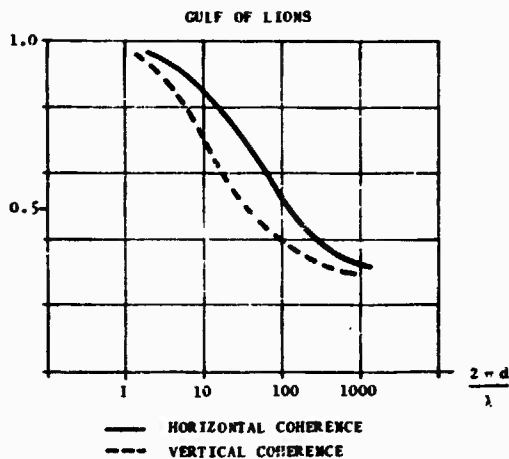
FIG. 4 SPATIAL COHERENCE MEASUREMENTS RESULTS, GULF OF LIONS
