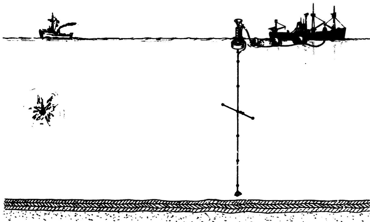
FIG. 1 EXPERIMENTAL ARRANGEMENT
