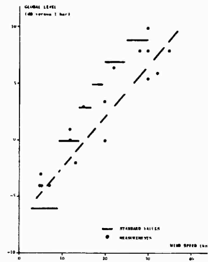
FIG. 3 MEASUREMENTS OF NOISE AS A FUNCTION OF WIND SPEED AND SEA STATE. GULF OF LIONS RESULTS
