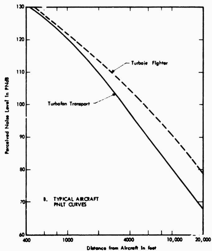
FIGURE 9. TYPICAL SOUND PROPAGATION CURVES
