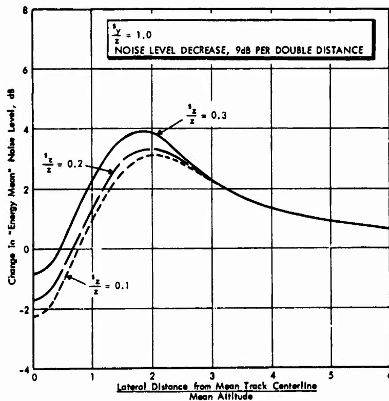
FIGURE 23. EFFECT OF FLIGHT PATH DISPERSION ON NOISE LEVELS FOR DIFFERENT DEGREES OF VERTICAL DISPERSION
