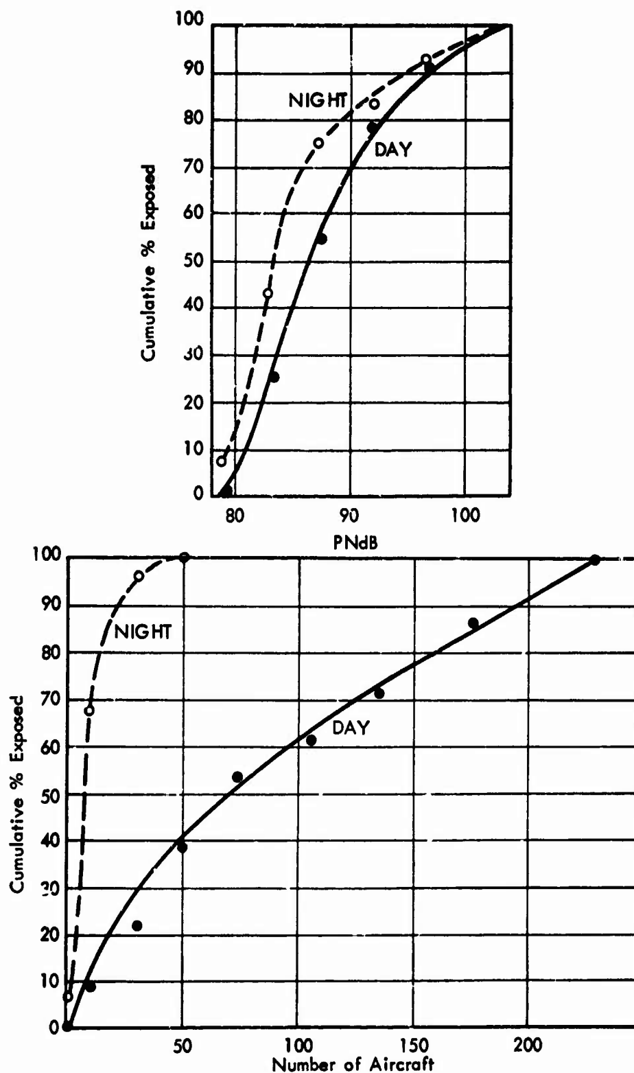
FIGURE 1. DAY AND NIGHT NOISE LEVELS AND NUMBER OF AIRCRAFT PRODUCING MORE THAN 80 PNdB OBSERVED IN 1967 LONDON SURVEY
