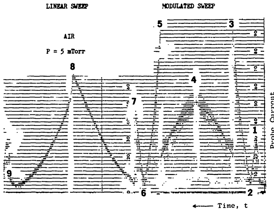
Fig. 12 — Recorder trace of the probe current in a plasma using pulsed and continuous sweeps
