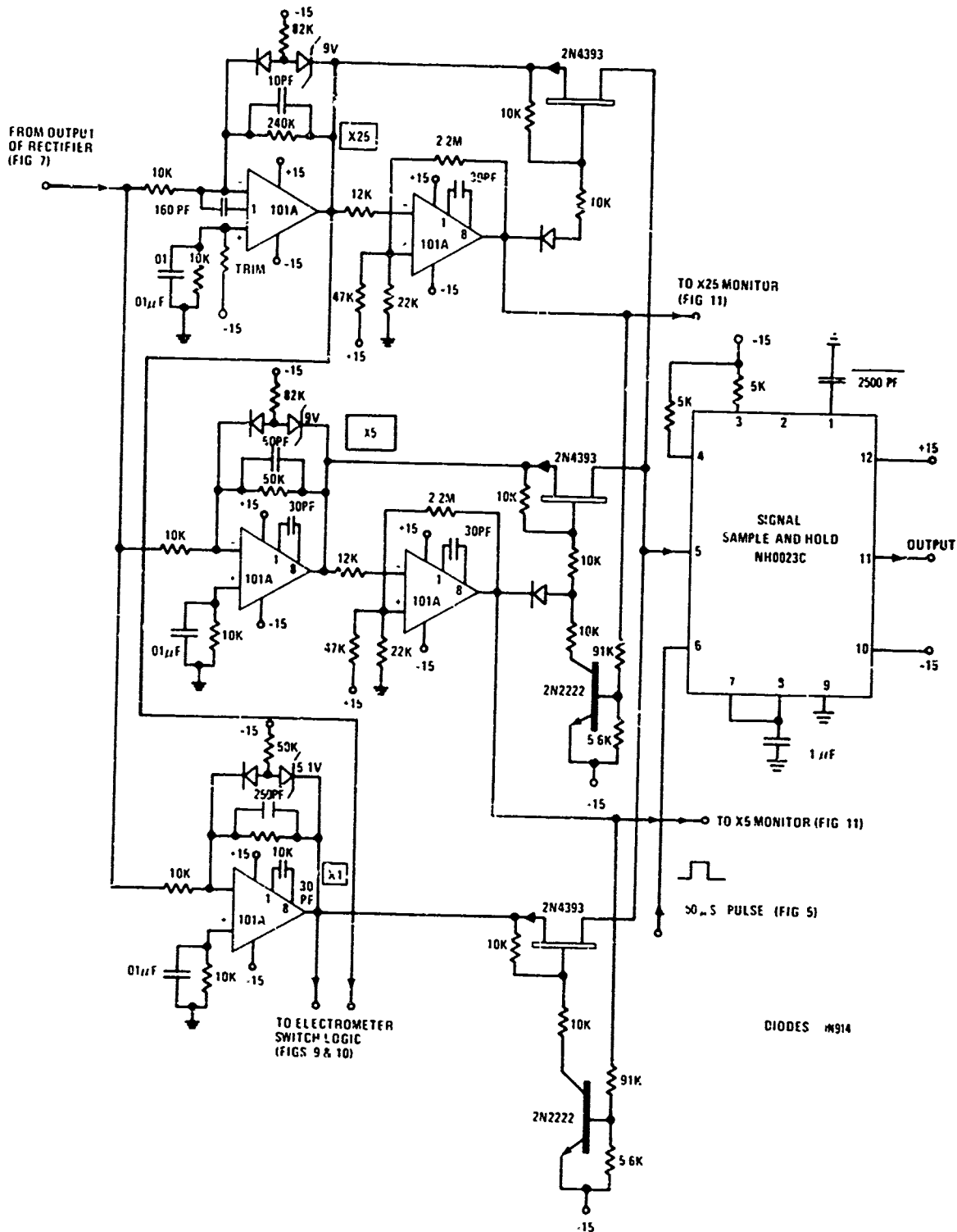
Fig. 8 - Scale charger
