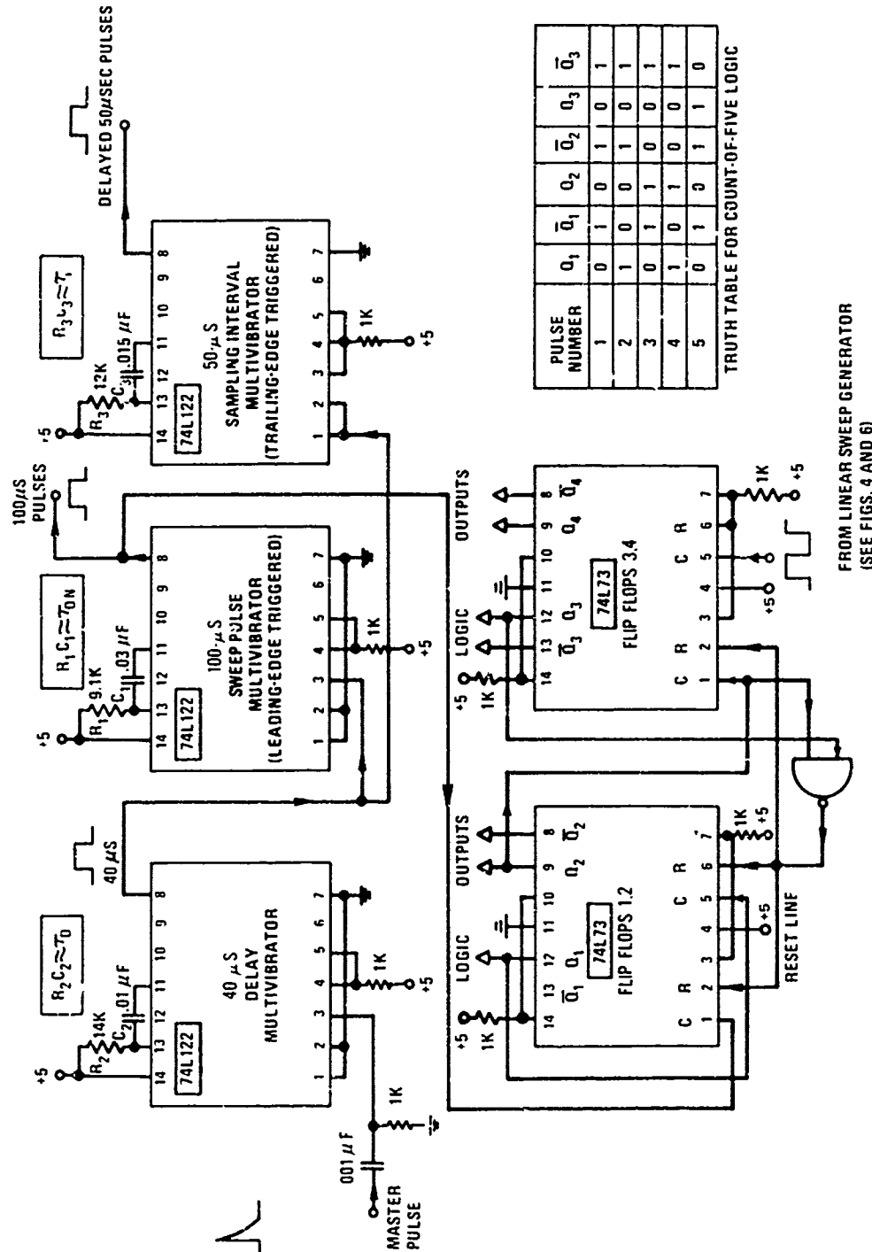
Fig. 5 — Multi-oscillators, count-of-five logic, and flip-flop 4. Arrows represent signal paths.
