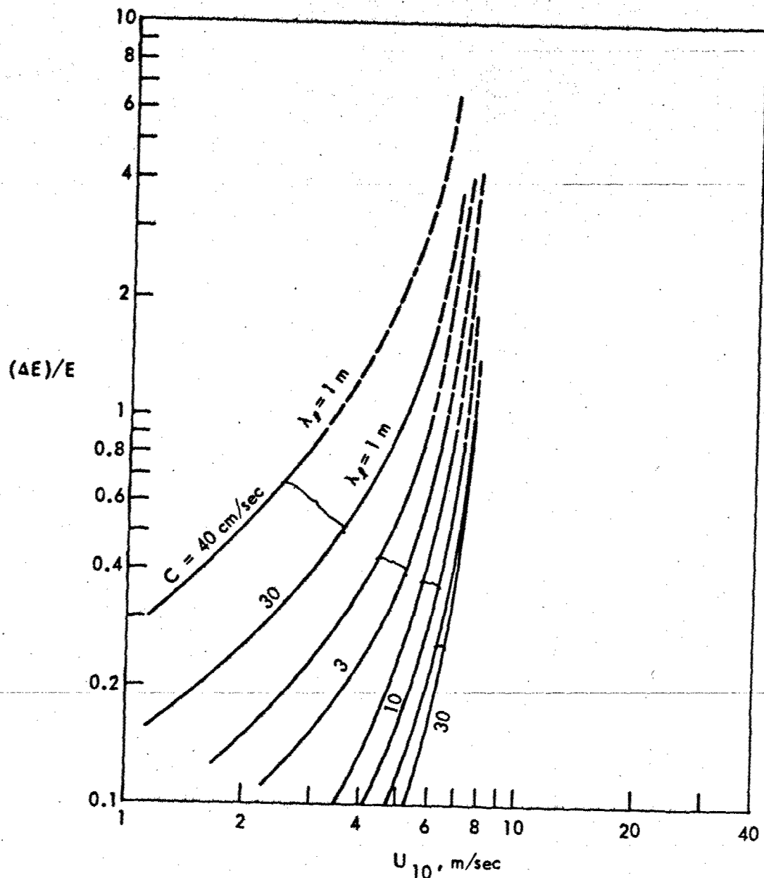
FIGURE 20 - PROPORTIONAL MODULATIONS IN ENERGY DENSITY OF SHORT BREAKING WAVES AS A FUNCTION OF WIND SPEED. Short wavelength \approx 2.5 \text{ cm} , surface current = 0, long wave slope = 0.2. The four pairs of curves, bracketed, are for long wavelengths of 1 meter, 3 meters, 10 meters, and 30 meters, the left-hand member of each pair being for an internal wave speed of 40 cm/sec, the other for 30 cm/sec.
