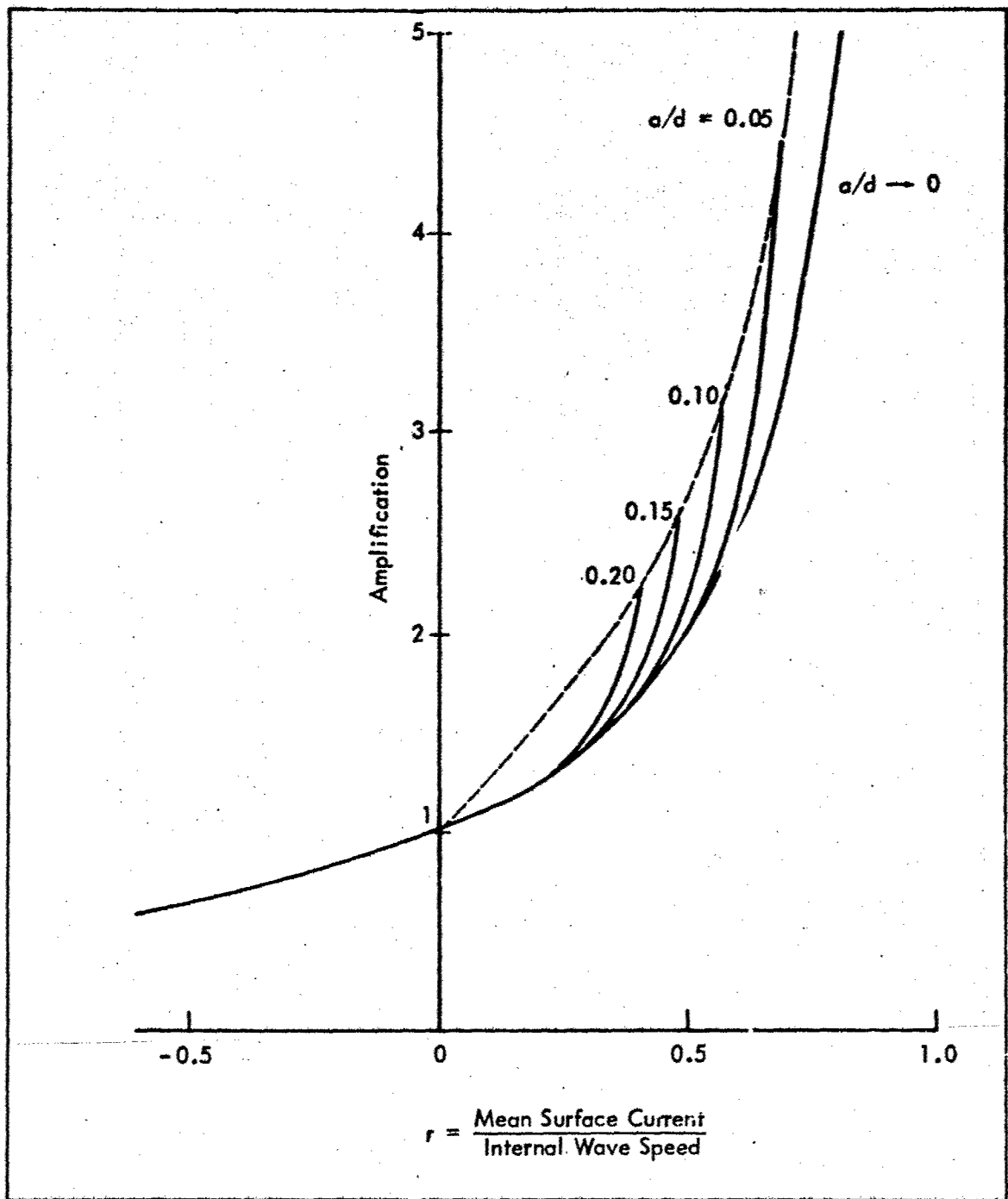
FIGURE 7 - THE AMPLIFICATION IN SURFACE CURRENT MODULATIONS RESULTING FROM THE EXISTENCE OF A MEAN CURRENT. Above the broken line, fluid at the surface above the internal wave troughs moves forward faster than the wave itself and a closed eddy forms.
