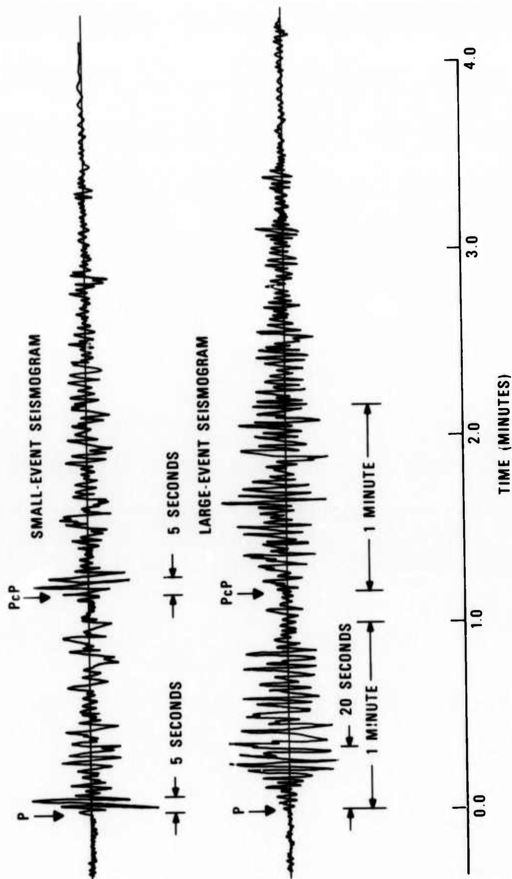
Figure 4. Hypothetical small-event and large-event seismograms.
