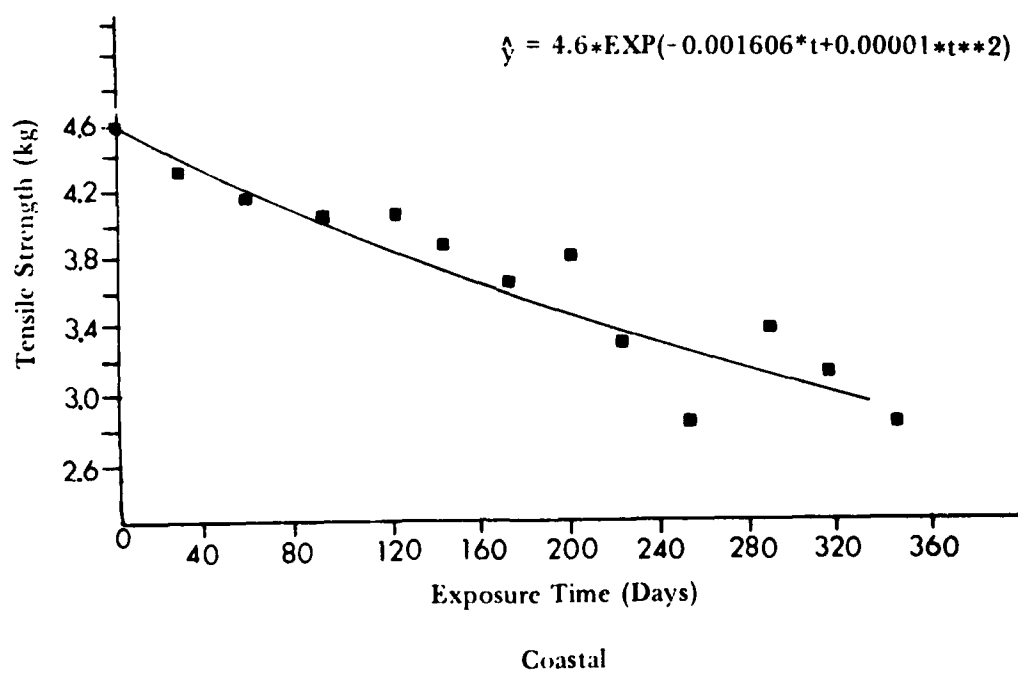
Figure C-4c and d. Exposure Modes for Polyvinyl Chloride Material.
