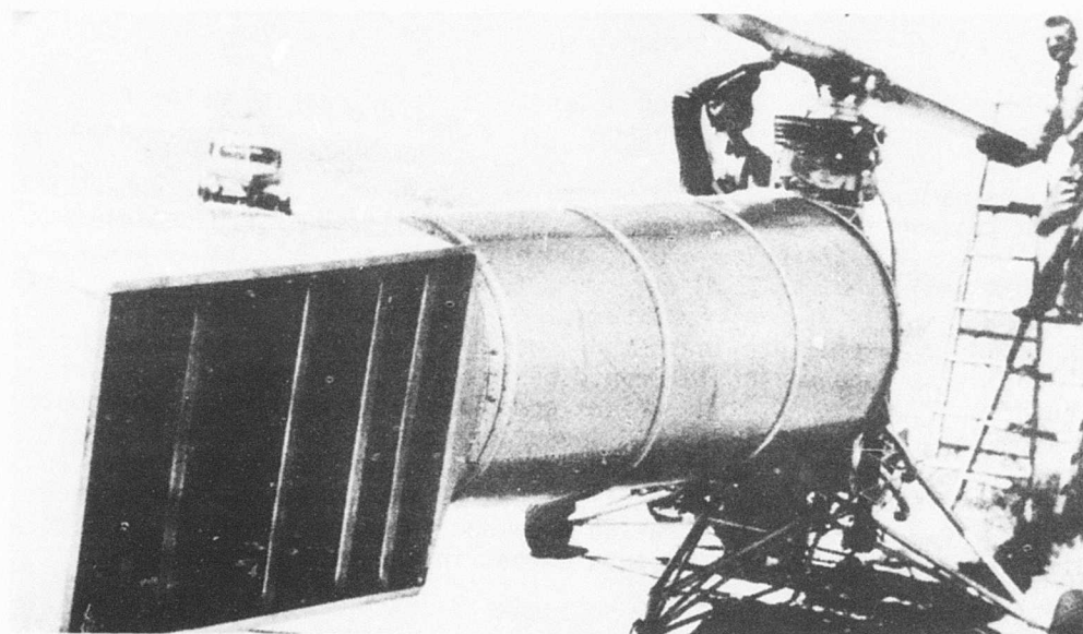
Hiller J-5
