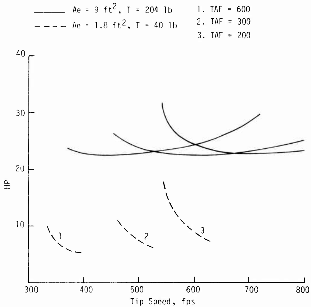
Figure 18. Fan Power Variation With Tip Speed and Total Activity Factor for C_1 = .5 and D_h/D_f = .3 .
