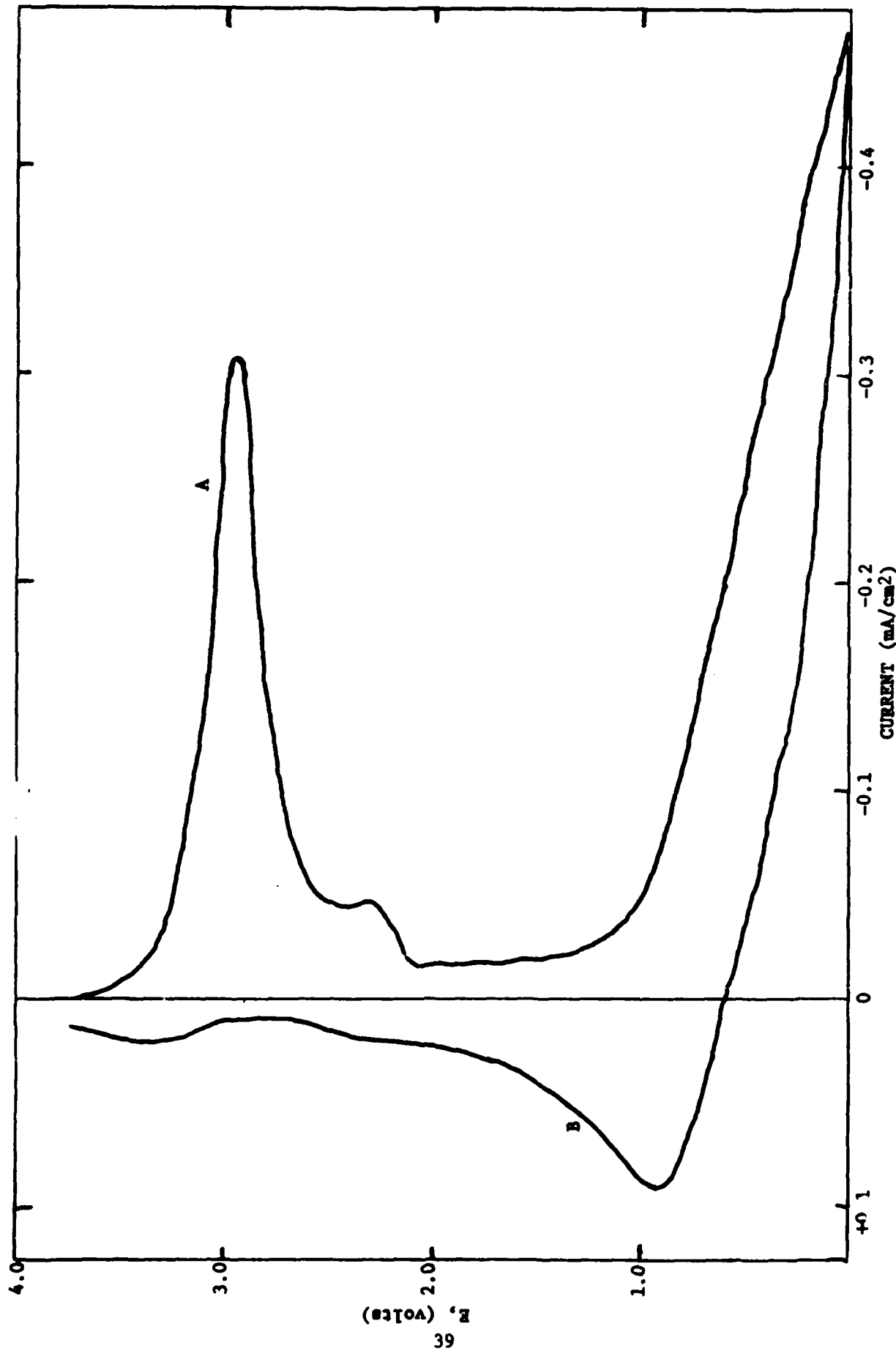
Fig. 18: Potentiostatic Reduction of \text{SOCl}_2 on Vitreous Carbon Stepping 100 mV/5 min. (A - cathodic scan, B - subsequent anodic scan)
