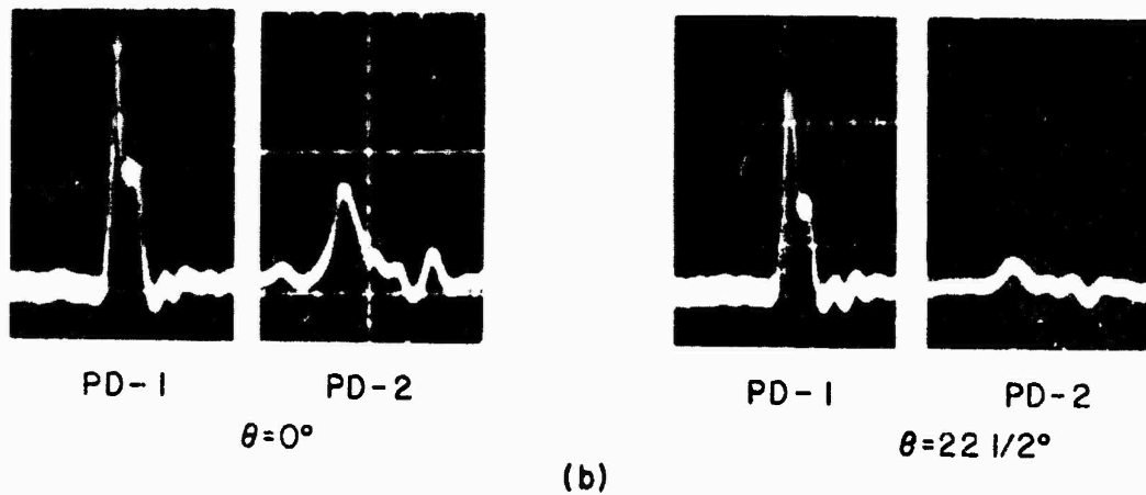
Fig. 2 — Measurements of Faraday rotation of specularly reflected light. (a) Arrangement for detecting the rotation of polarization. Arrows indicate the directions of polarization (mutually perpendicular). The whole detector can be rotated by an angle \theta . (b) Photodiode outputs for detector assembly set at \theta = 0 (left) and at \theta = 22\frac{1}{2}^\circ (right).
