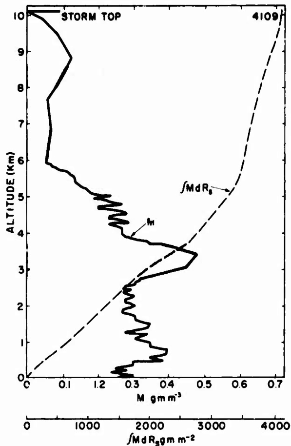
Figure 4. Profiles of Liquid-Water-Content, M , and Integral of Liquid-Water, \int M dR_s , for the Missile Trajectory
