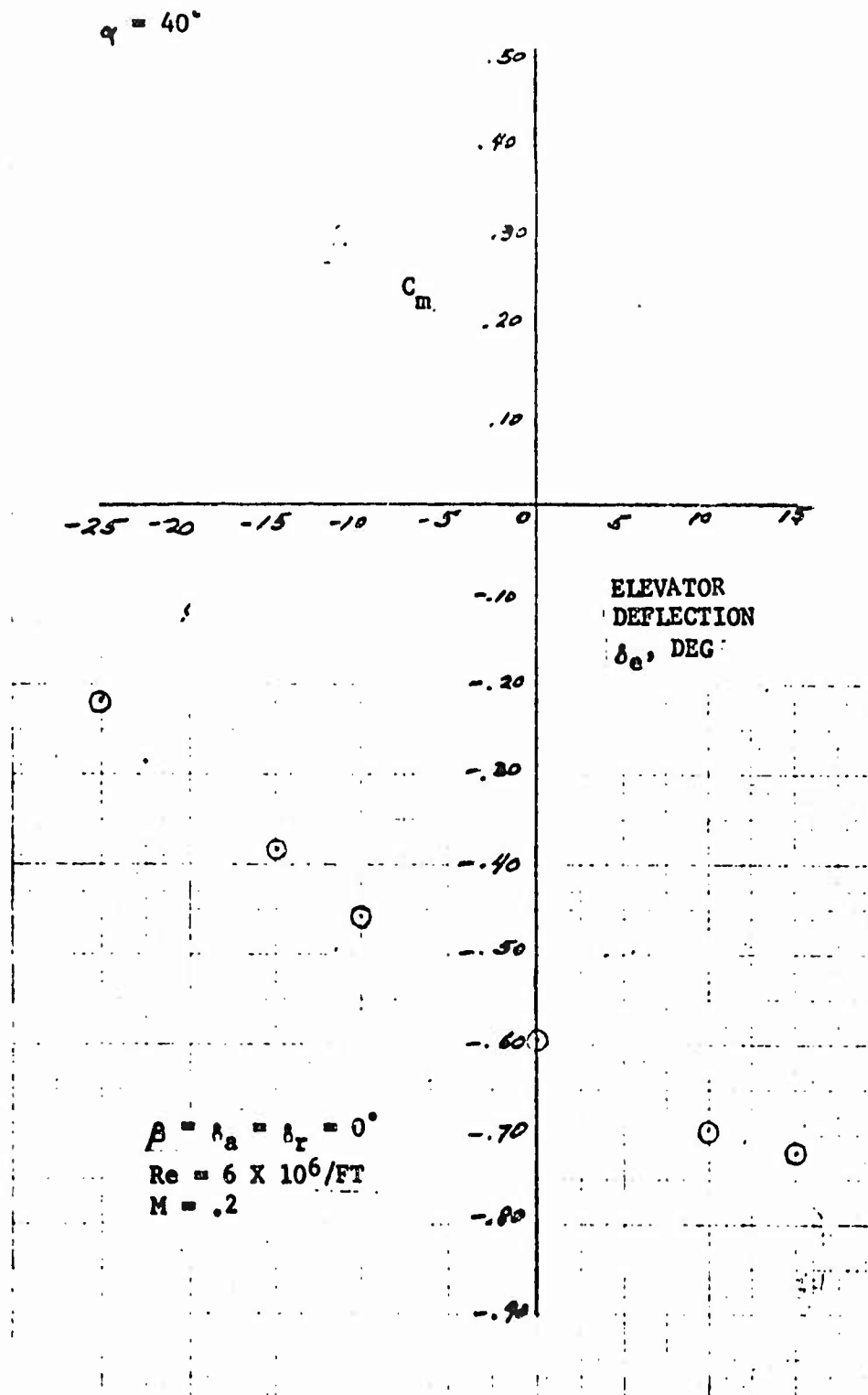
FIGURE 39. COEFFICIENT OF PITCHING MOMENT VERSUS ELEVATOR DEFLECTION FOR VARIOUS ANGLES-OF-ATTACK (CONT)
