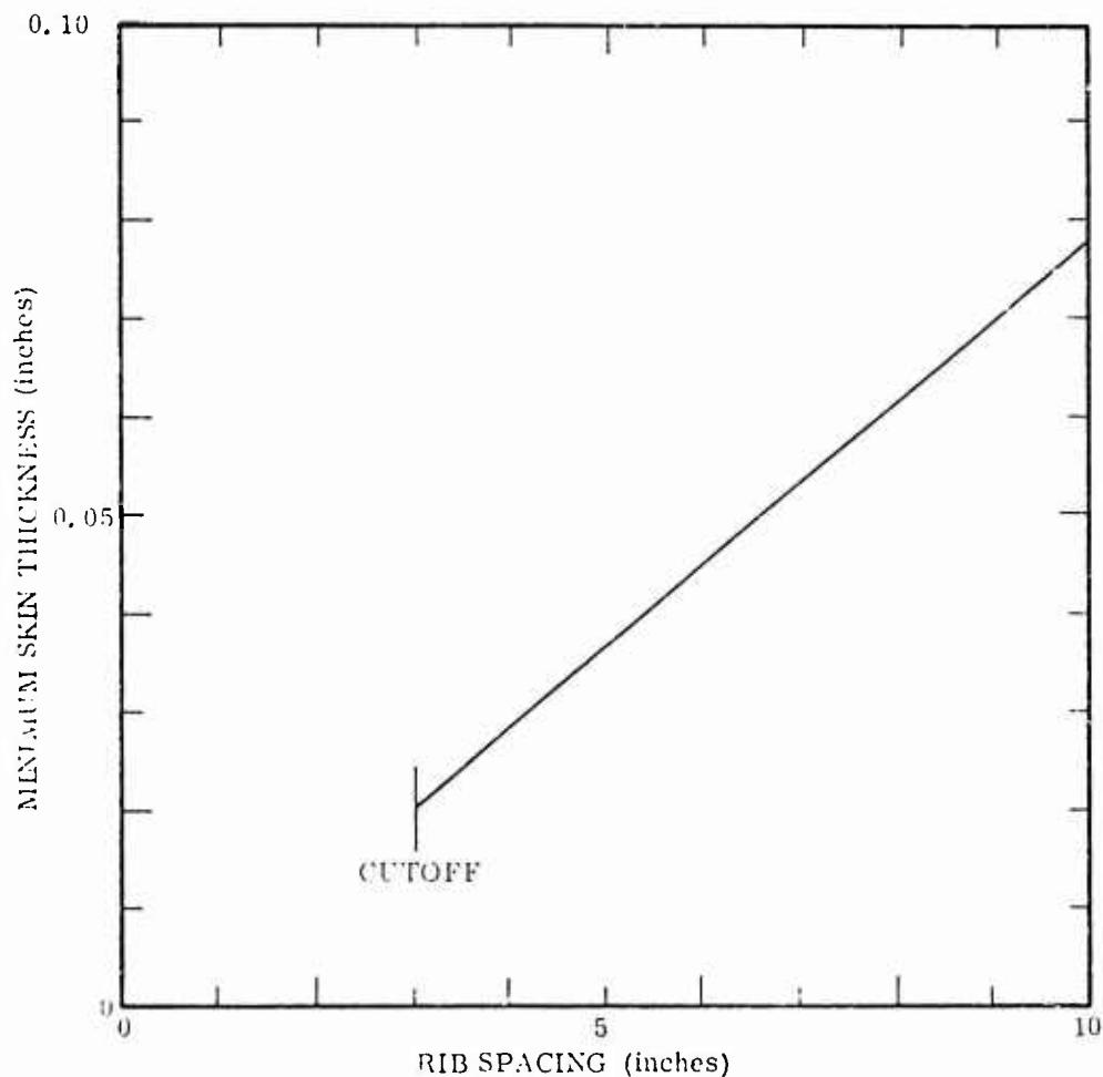
Figure 19. Sonic Fatigue Curve.
