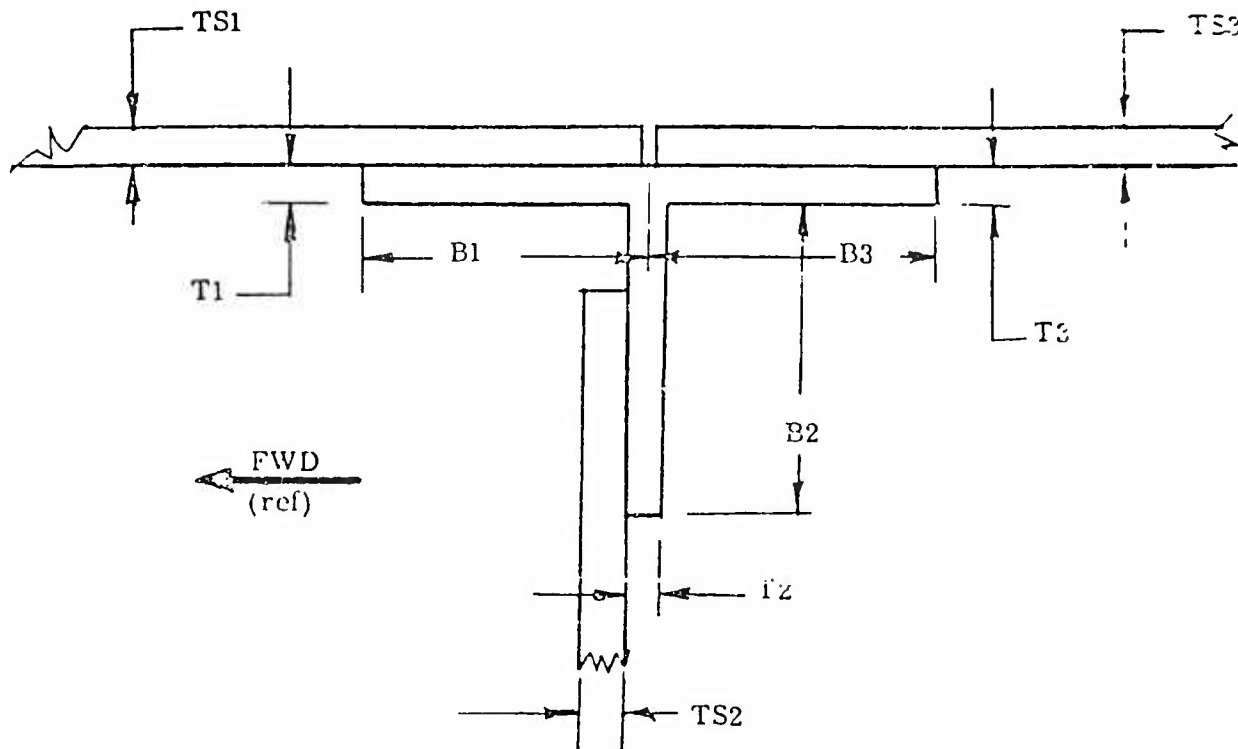
Figure 9. Typical Spar Cap Model - Built Up Web.
