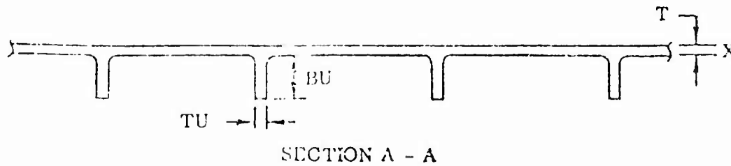
Figure 11. Integral Web.
