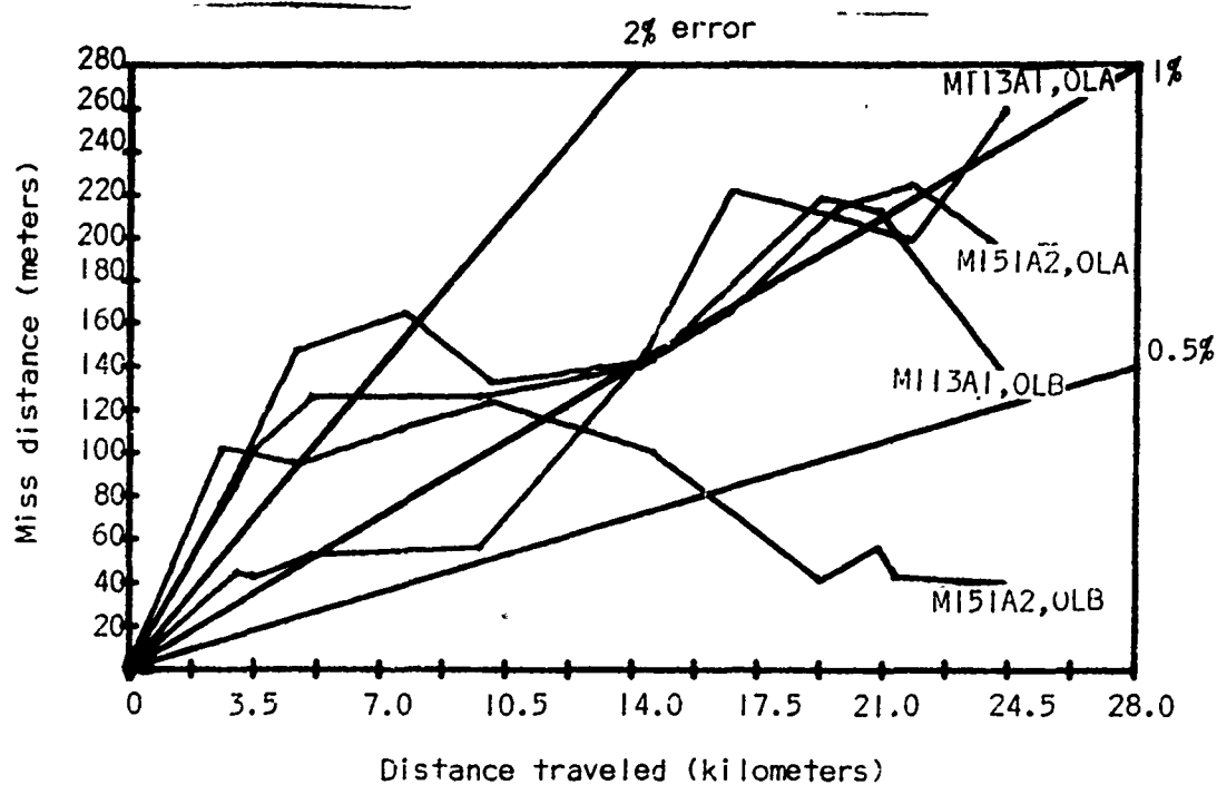
Figure D-9. Average miss distance and percent error for distance traveled for the LNS-518 vehicle navigation system mounted in an MI13A1, and MI51A2 on the open level course traveling clockwise (OLA) and counterclockwise (OLB).
