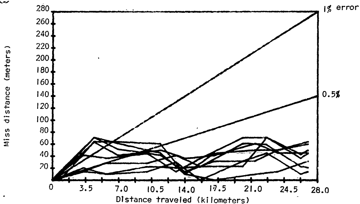
Figure 6-13. Miss distance and runs conducted by the AGA vehicle navigation system mounted in the MI51A2 traversing open end, level course.
