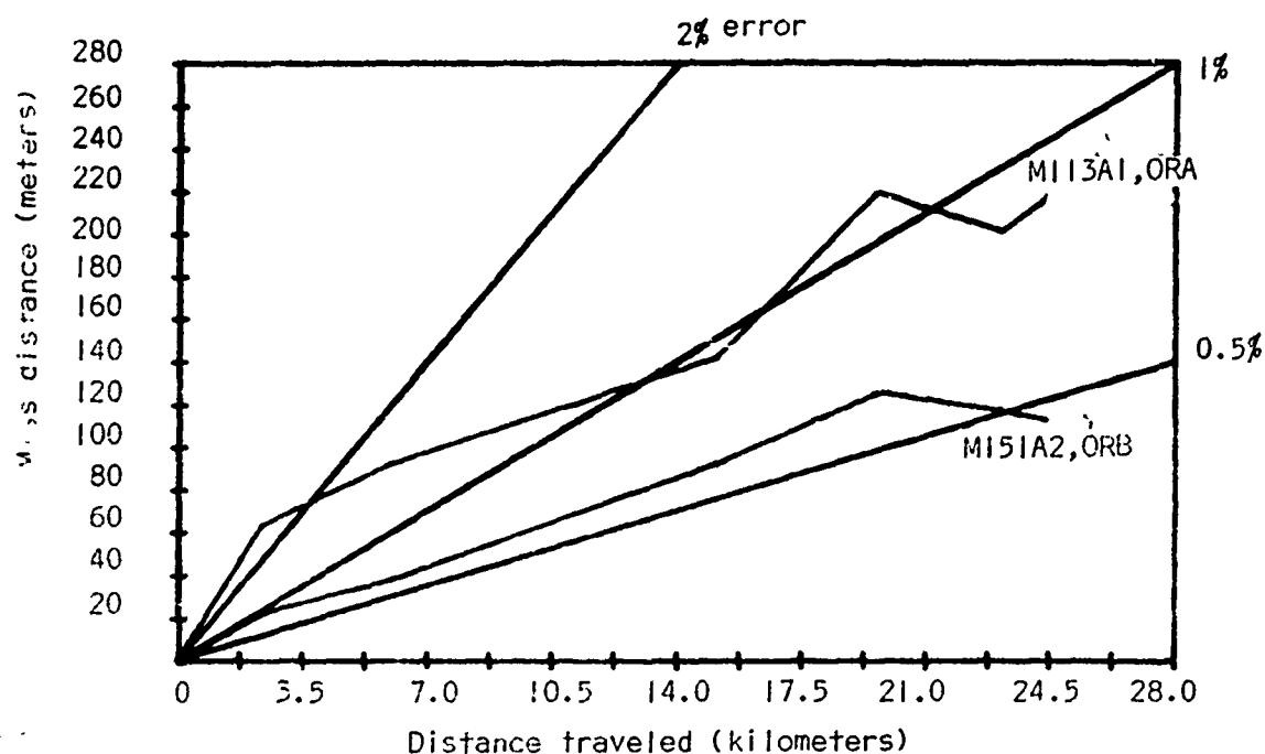
Figure D-8. Average miss distance and percent error for distance traveled for the LNS-518 vehicle navigation system mounted in an MI13A1 on the open rough course traveling clockwise (ORA), and MI151A2 traveling counterclockwise (ORB).
