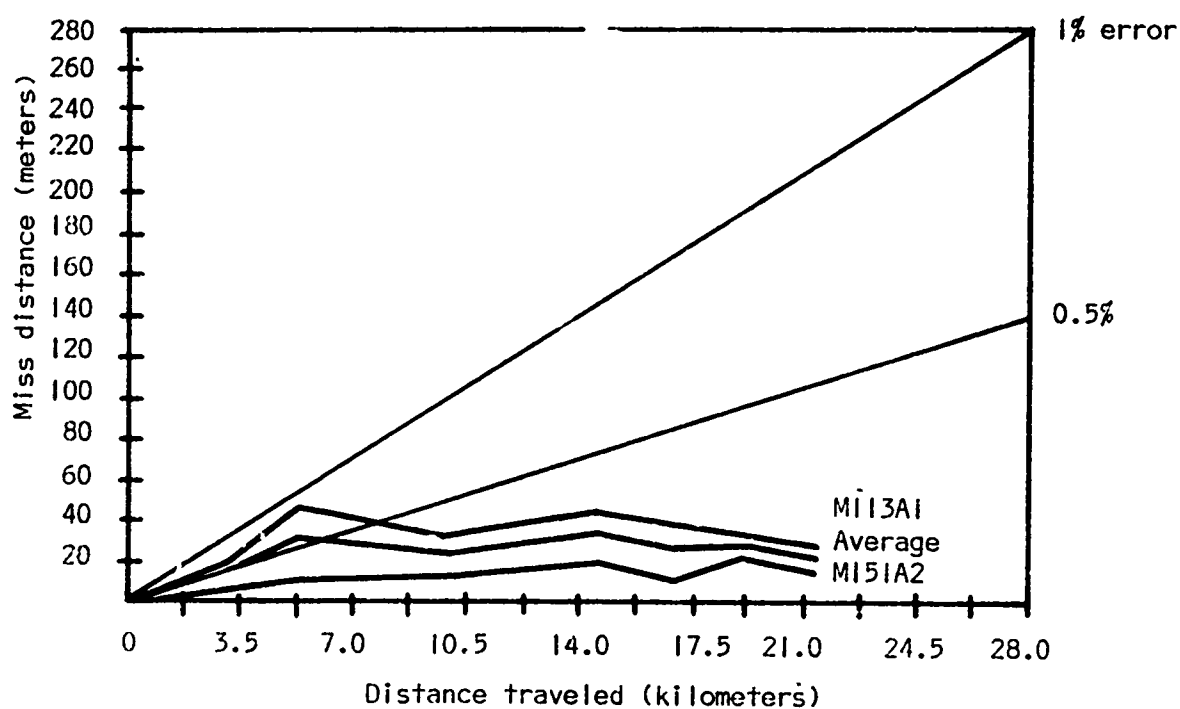
Figure C-22. Average miss distance and percent error for distance traveled for the AGA vehicle navigation system mounted in an M113A1 and M151A2; and the system average for the closed level course traveling clockwise.
