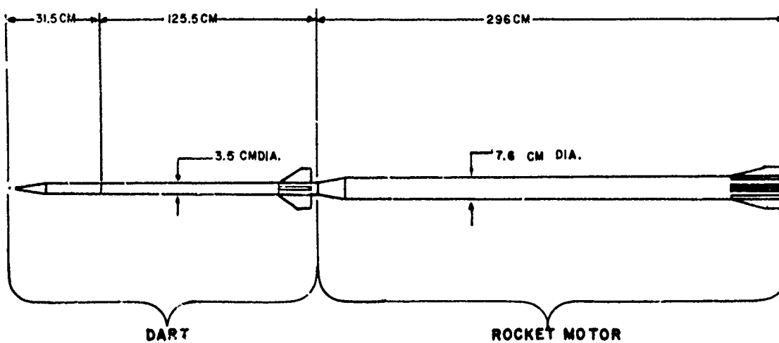
Figure 2. Loki dart vehicle configuration (assembled weight: 15.4 kg).
