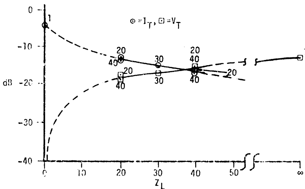
FIGURE 75 MODE 1 INPUT \Delta TRANS. TF1010 SHIELD ON OUTPUT Y PULSE P5
