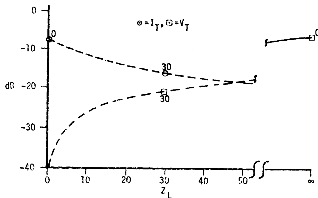
FIGURE 76 MODE 2 INPUT Y TRANS. TF1010 SHIELD ON OUTPUT \Delta PULSE P4
