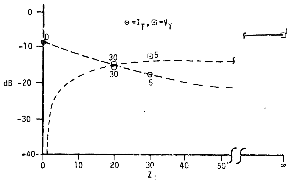
FIGURE 42 MODE 2 INPUT Y TRANS. TFAA/FA SHIELD ON OUTPUT Δ PULSE P5
