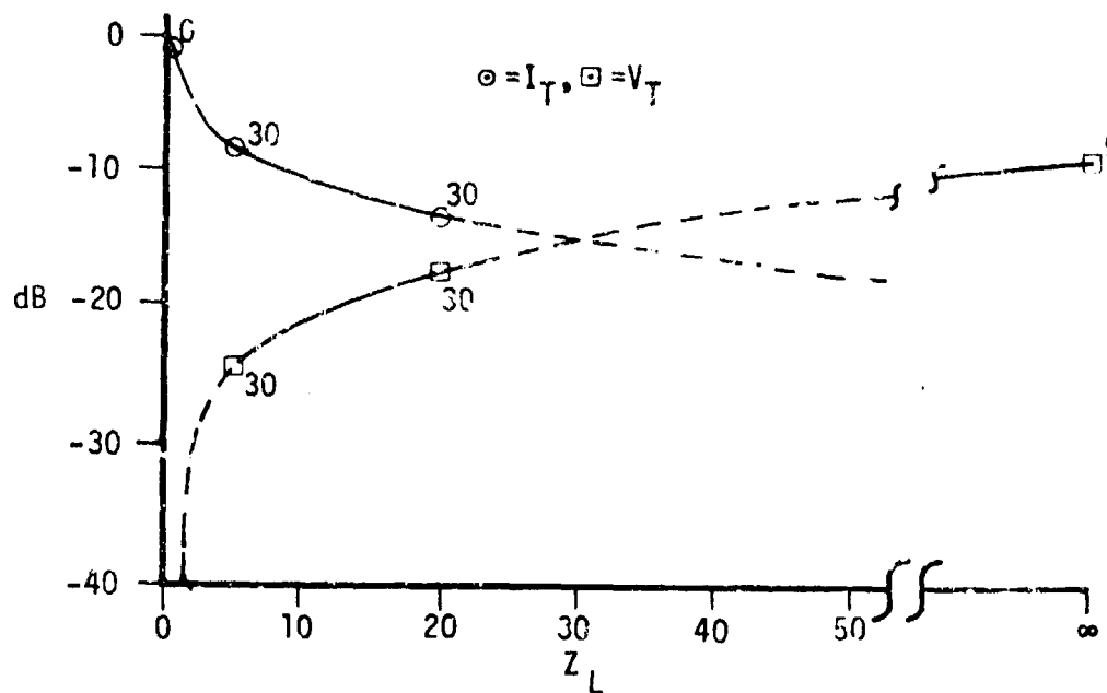
FIGURE 43 MODE 2 INPUT Δ TRANS. TFAA/FA SHIELD ON OUTPUT Y PULSE P5
