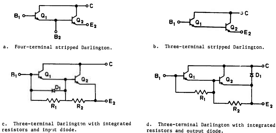
Figure 20. Commercially available Darlington circuits.
