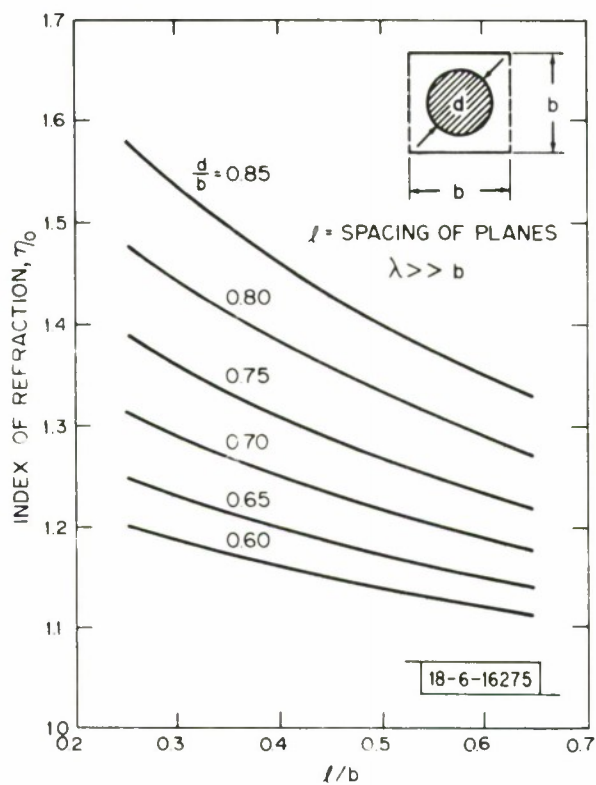
Fig. 5. Electrolytic tank measured values for a square distribution of circular disks.
