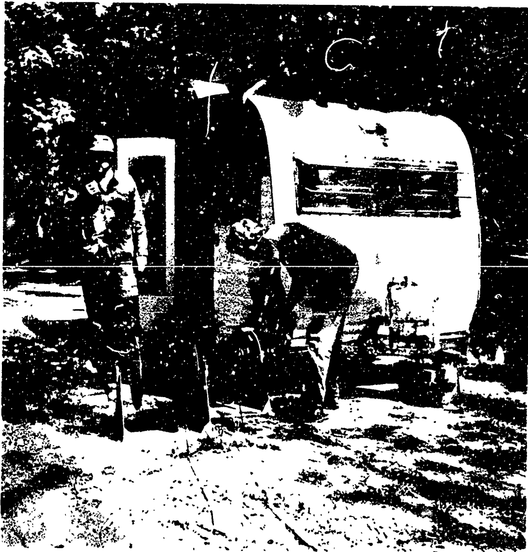
Figure 9. Two 1000' reels of coax cable connecting photocon microphones to measuring and recording equipment installed in the 12' mobile camper-trailer.
