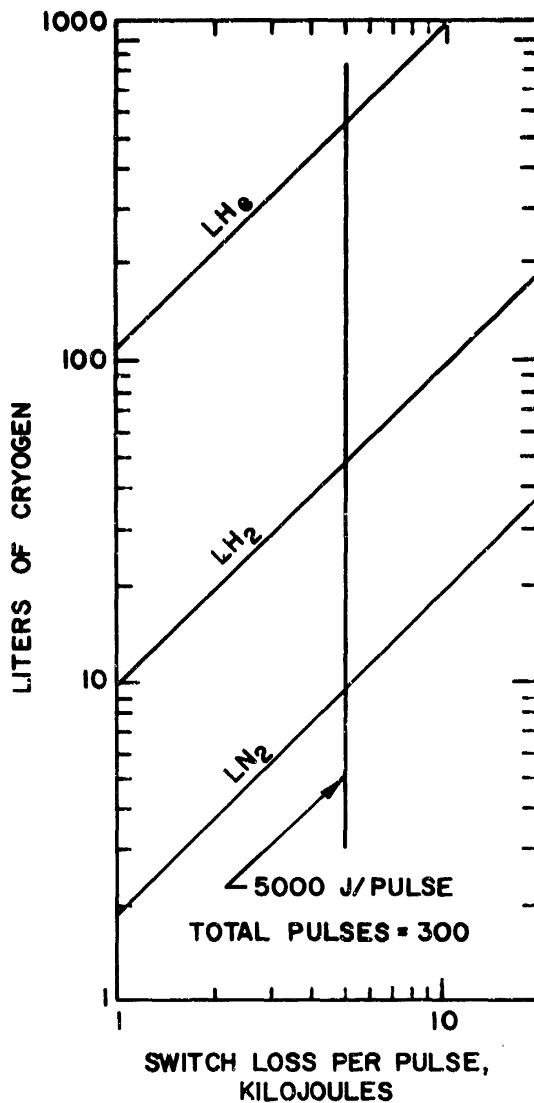
Figure 9. Liquid liters of cryogen necessary to support switch losses (estimates based on heat of vaporization only).
