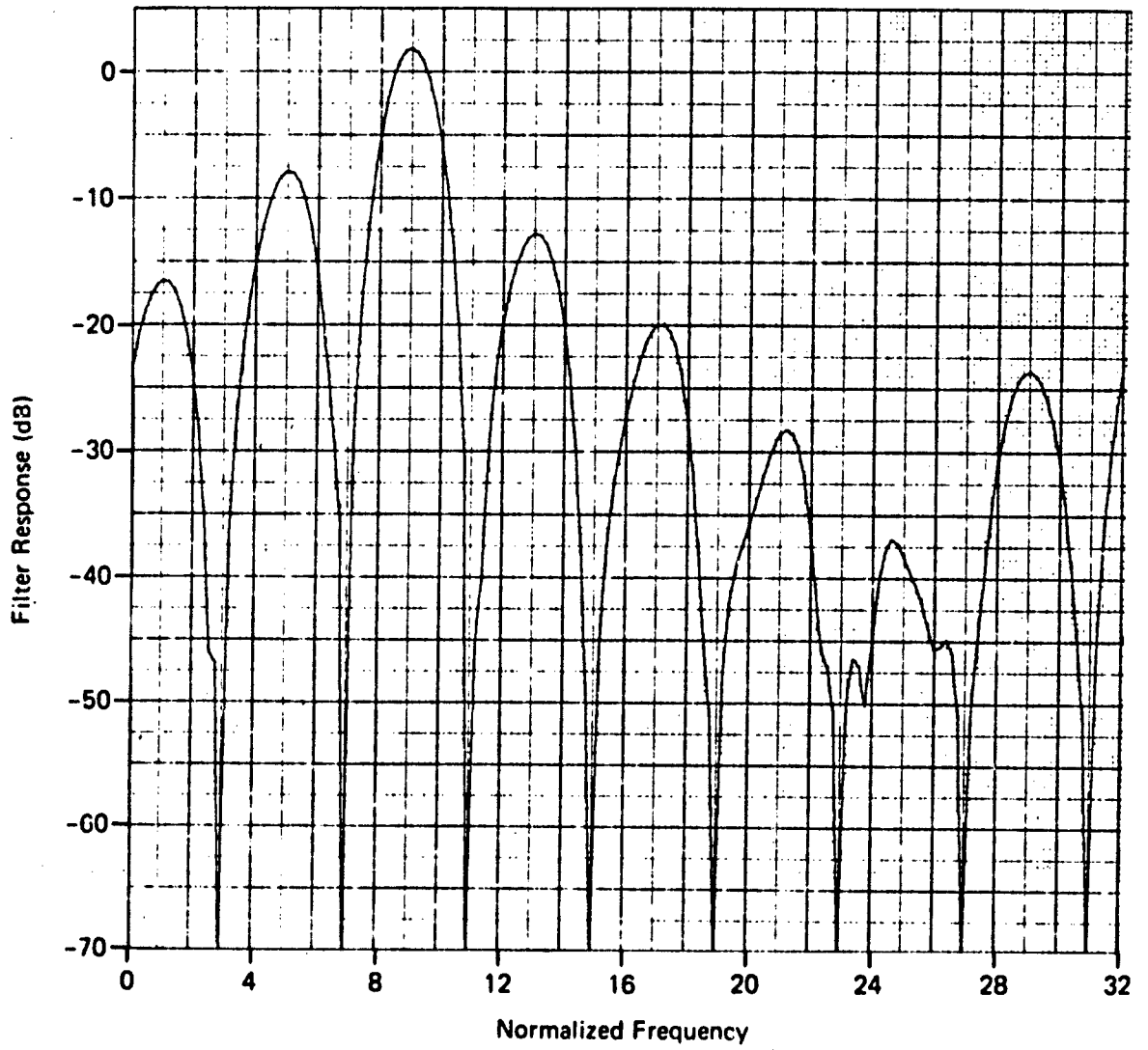
Fig. 21 Hamming Weighting 0-bit Fourier Processing; N = 32 , f_0 = 9
