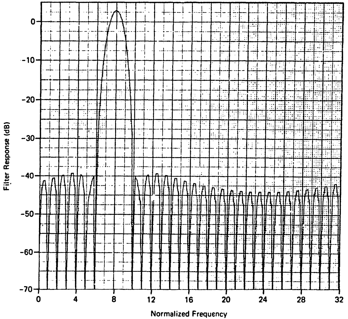
Fig. 10 Hamming Weighting Walsh Processing; N = 32 , f_0 = 8
