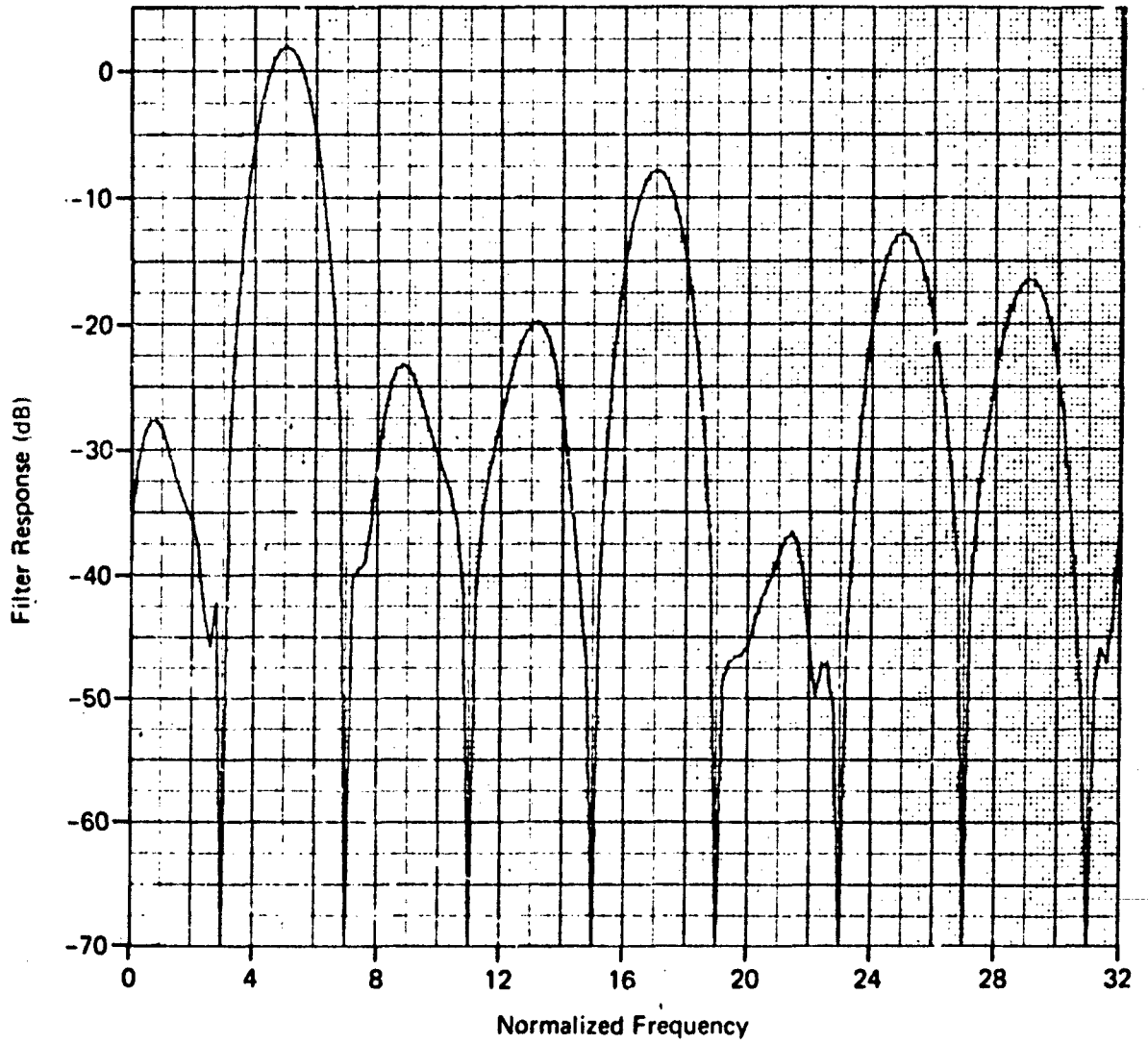
Fig. 19 Hamming Weighting 0-bit Fourier Processing; N = 32 , f_0 = 5
