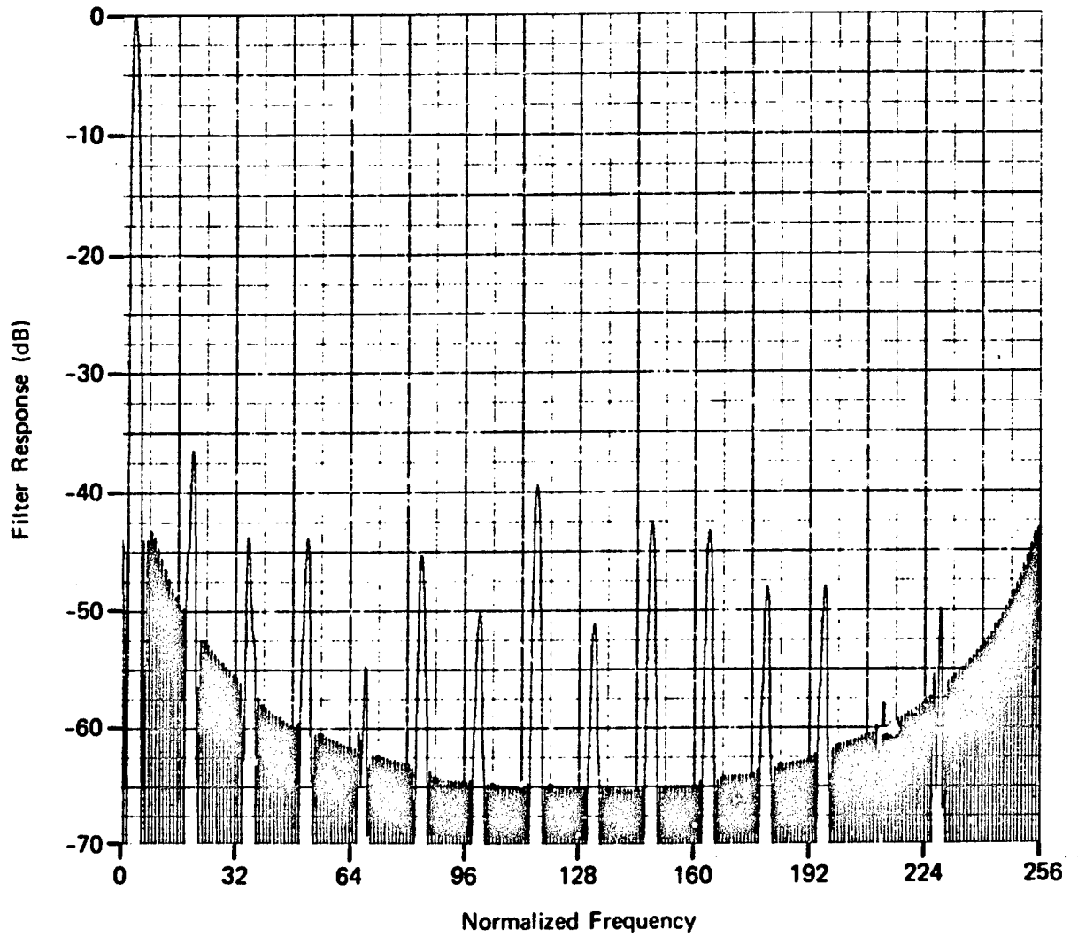
Fig. 37 Hamming Weighting 4-bit Fourier Processing; N = 256 , f_0 = 4
