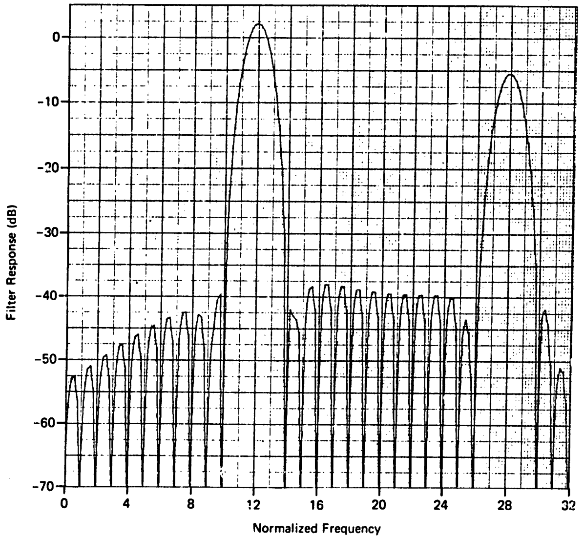
Fig. 12 Hamming Weighting Walsh Processing; N = 32 , f_0 = 12
