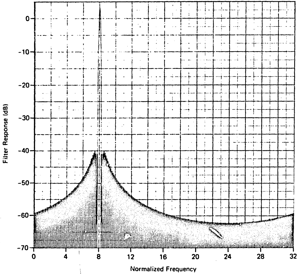
Fig. 36 Hamming Weighting Walsh Processing; N = 256 , f_0 = 64
