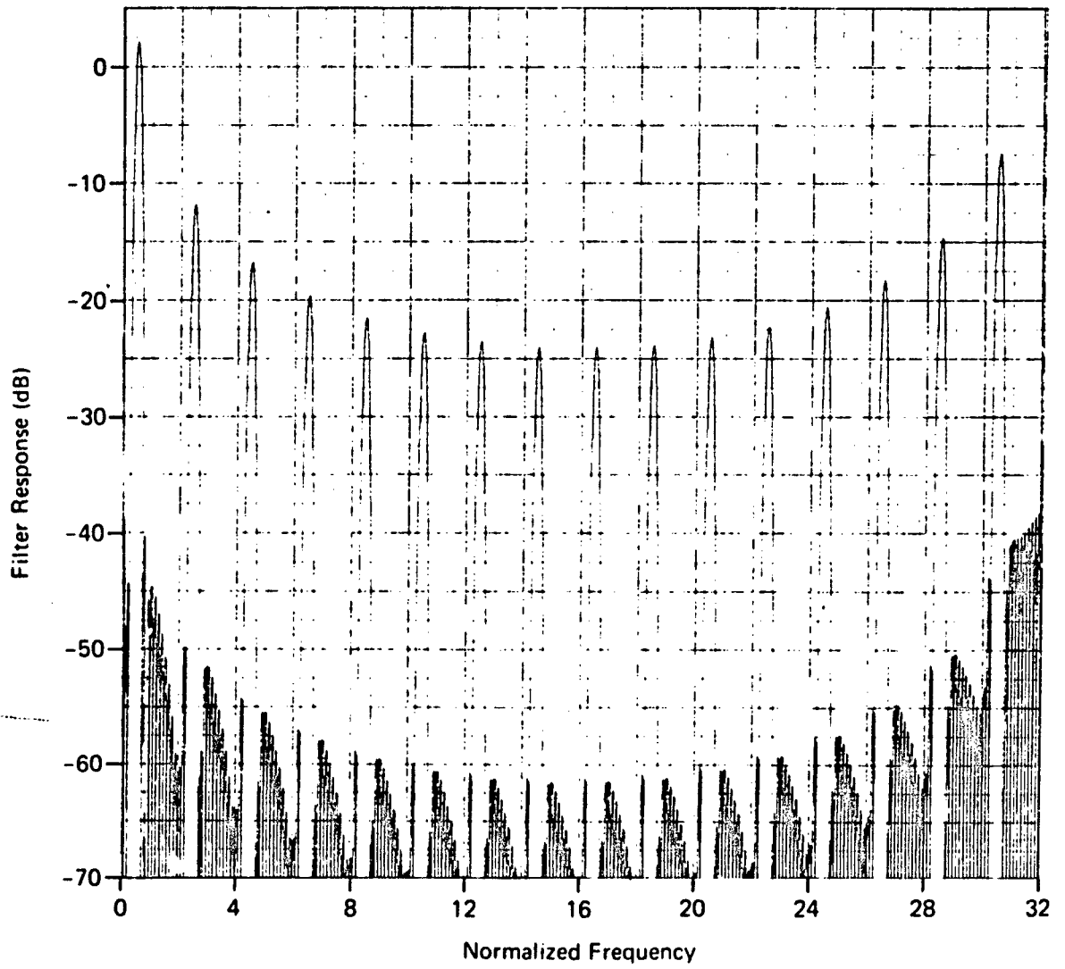
Fig. 32 Hamming Weighting Walsh Processing; N = 256 , f_0 = 4
