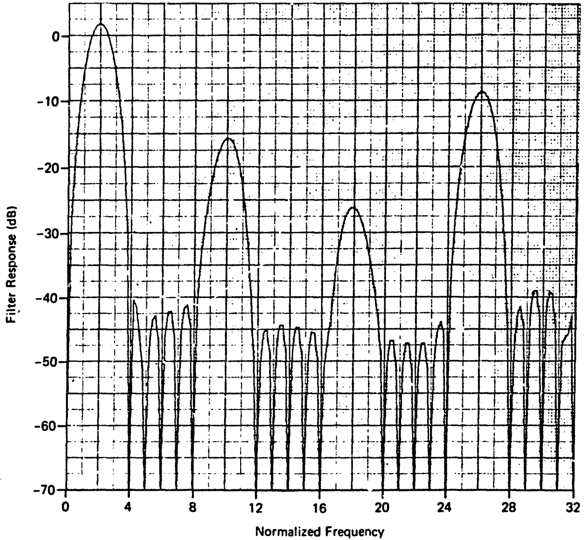
Fig. 16 Hamming Weighting 0-bit Fourier Processing; N = 32 , f_0 = 2
