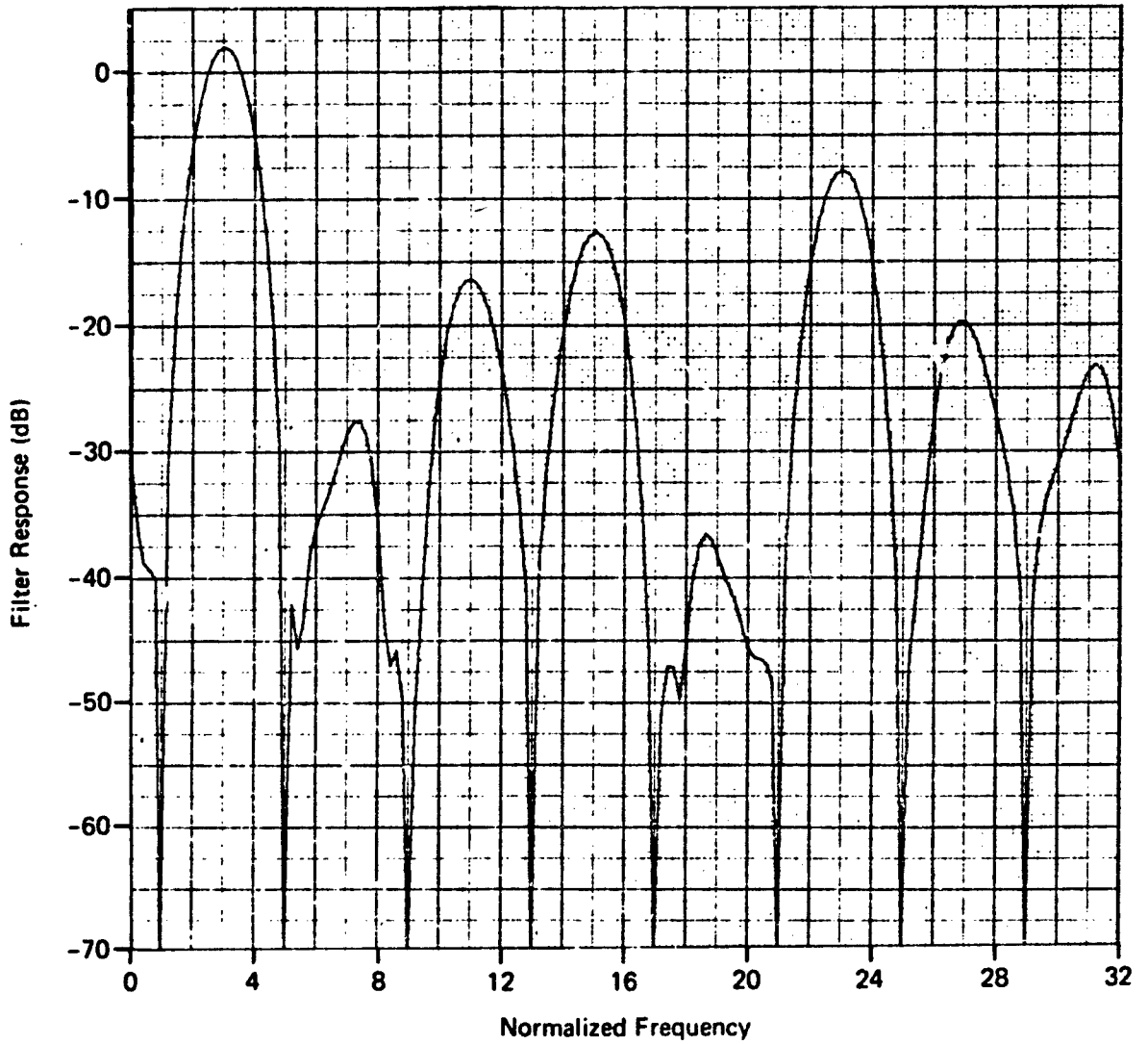
Fig. 17 Hamming Weighting 0-bit Fourier Processing; N = 32 , f_0 = 3
