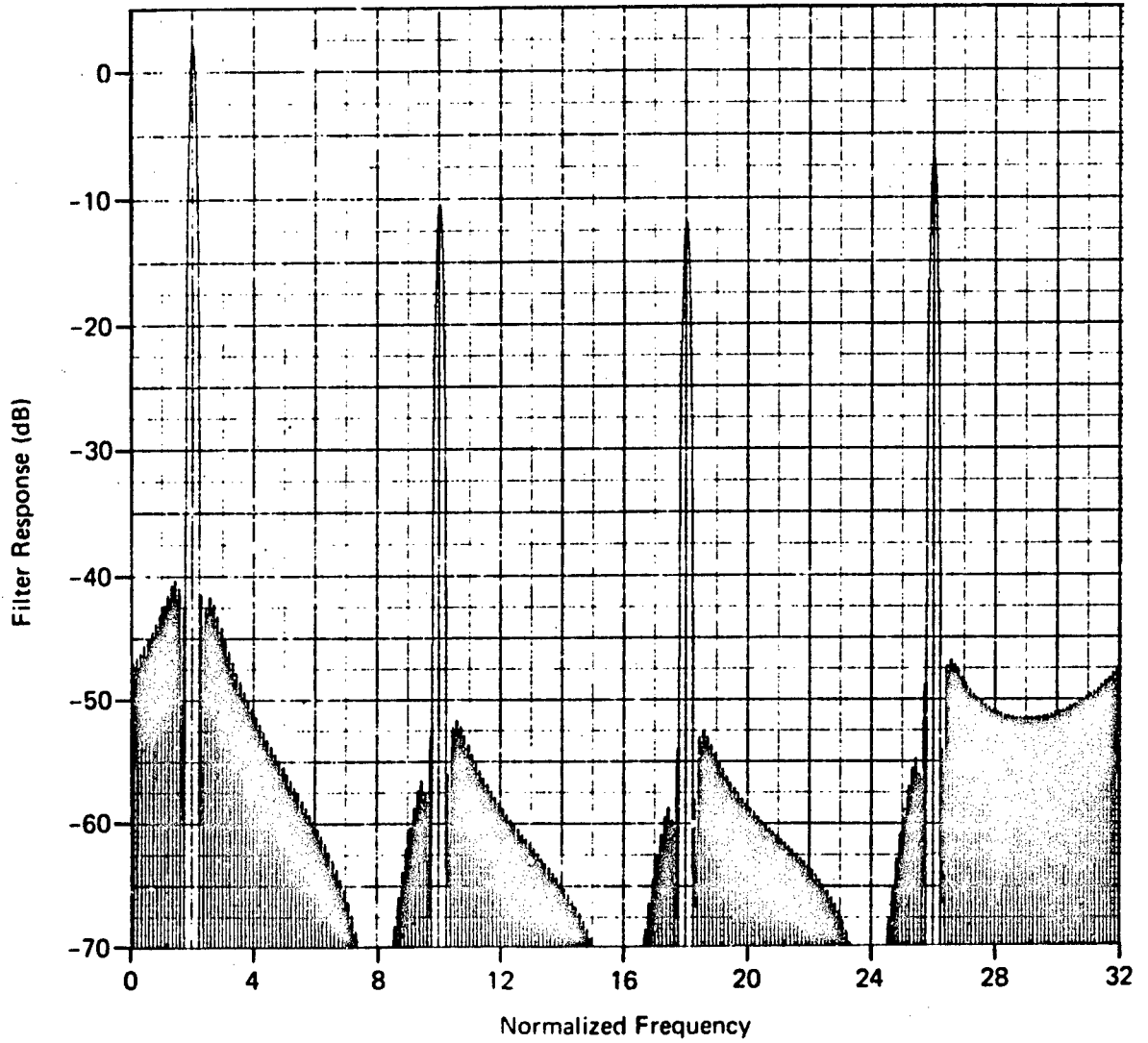
Fig. 34 Hamming Weighting Walsh Processing; N = 256 , f_0 = 16
