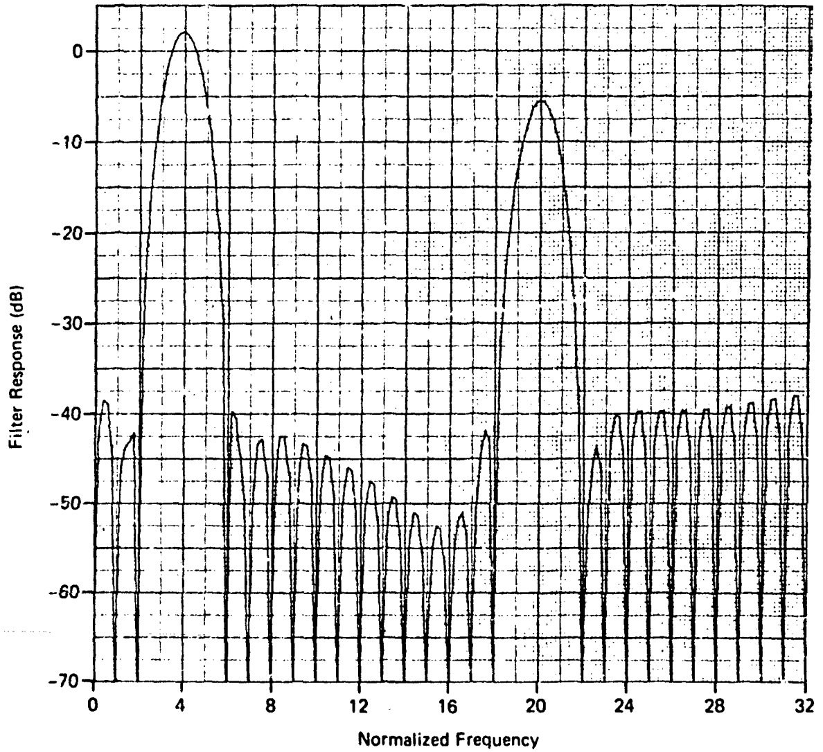
Fig. 7 Hamming Weighting Walsh Processing; N = 32 , f_0 = 4
