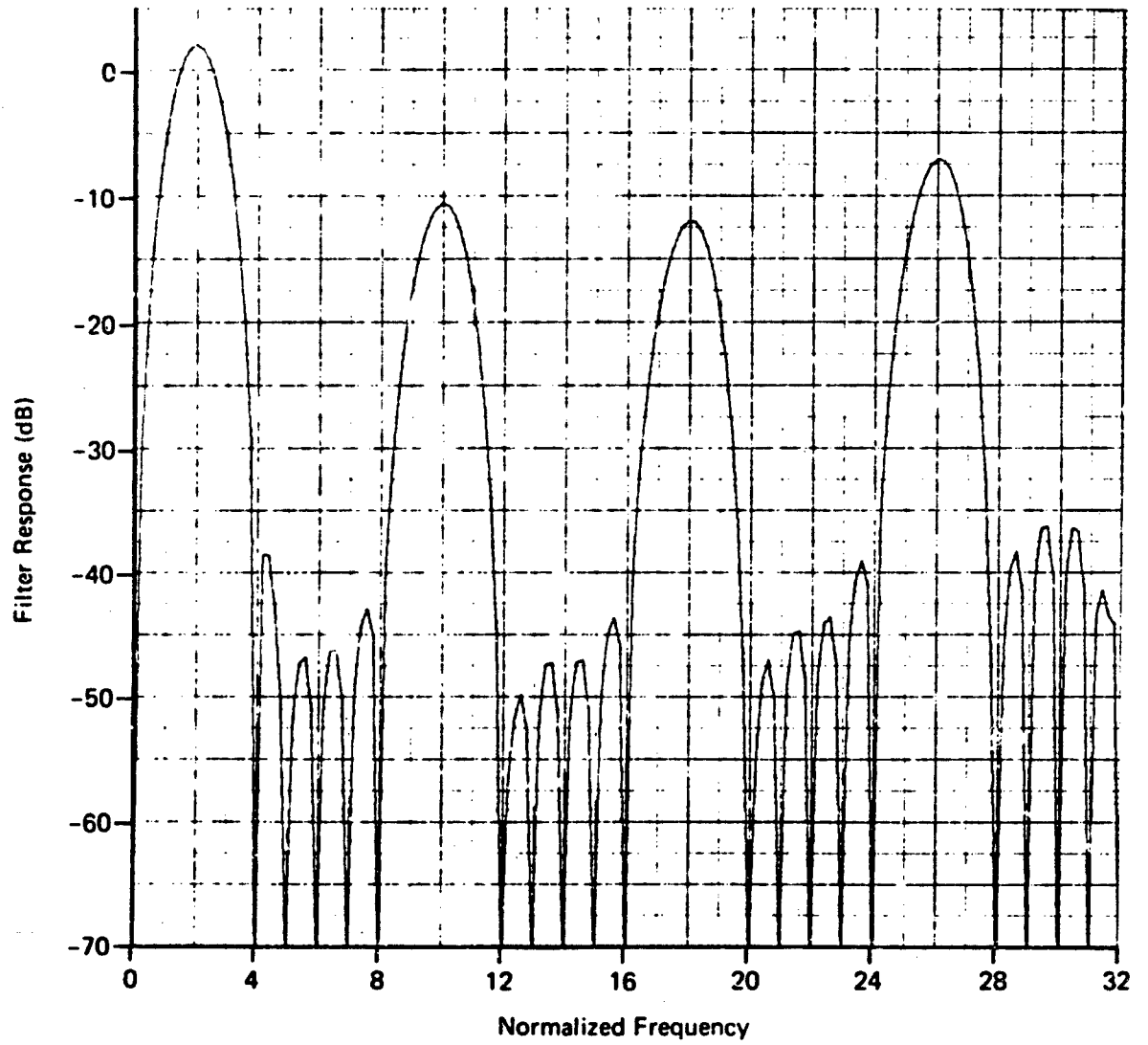
Fig. 5 Hamming Weighting Walsh Processing; N = 32 , f_0 = 2
