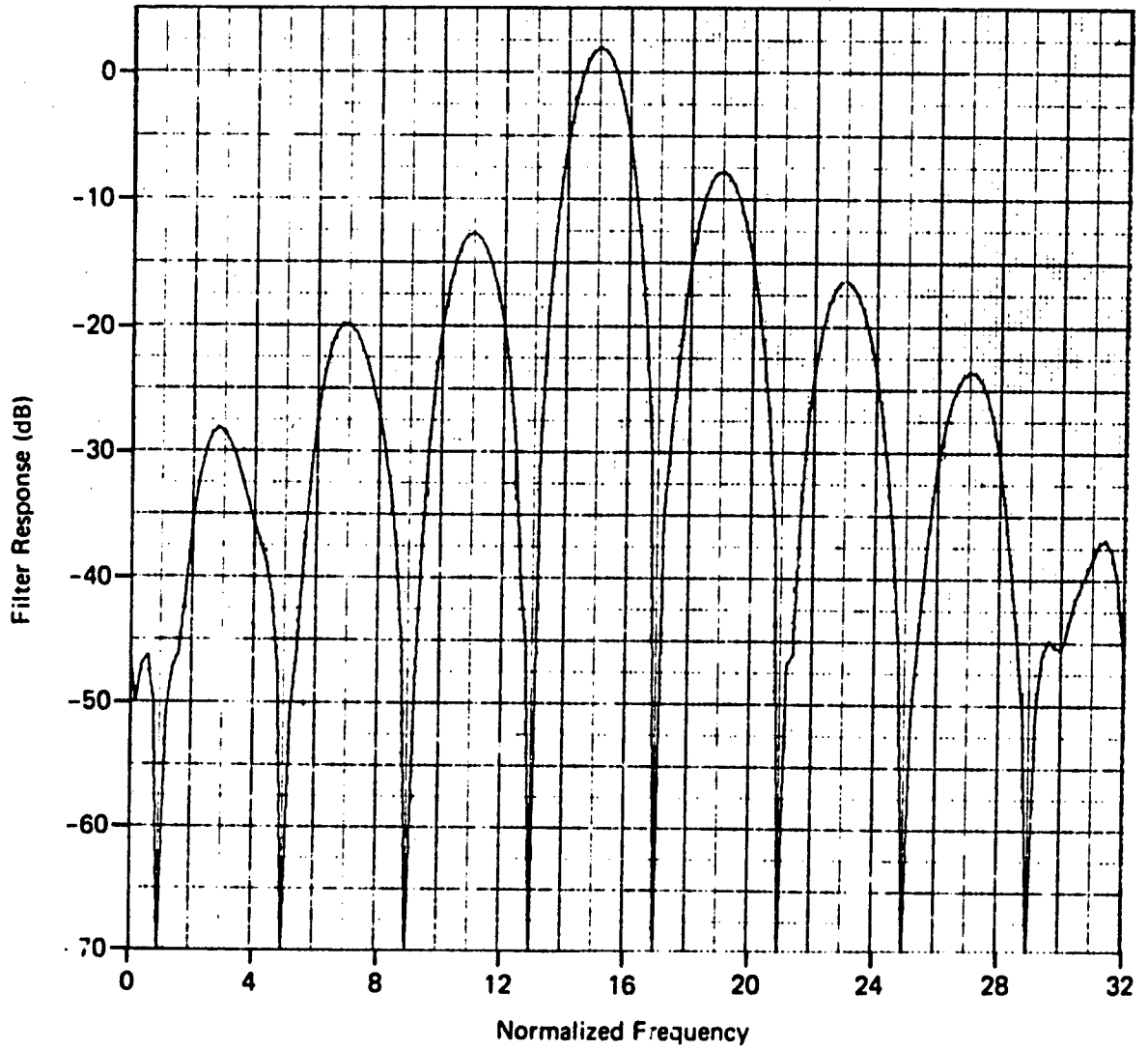
Fig. 23 Hamming Weighting 0-bit Fourier Processing; N = 32 , f_0 = 15
