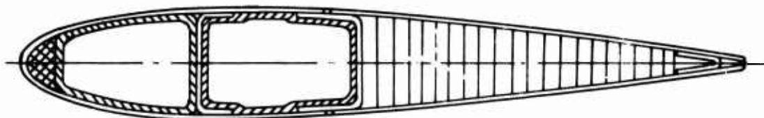
CONCEPT D – METAL AND COMPOSITE BLADE
