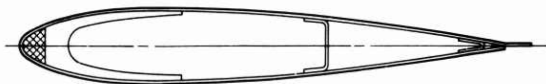
CONCEPT A – OH-6A ALUMINUM BLADE
