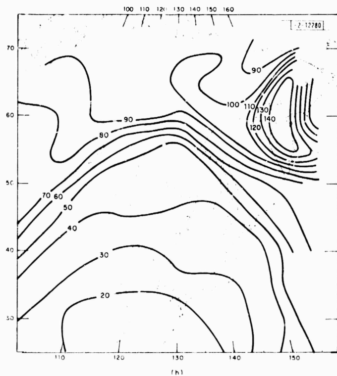
Fig. 11-1. Standard error (km) of focal depths computed using P-waves only from DARPA seismic network assuming standard error of each arrival time of 1.0 s.c. (a) Eastern half of Eurasia; (b) western half of Eurasia.
