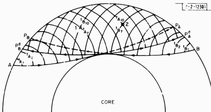
Fig. IV-7. Shadow zones for two events >95^\circ apart. Rays P_A and P_B define strictly geometrical shadow zones for events at points A and B. Rays P_A^d and P_B^d are typical paths for diffracted P-waves from these sources. Arcs represent position of P-wave wavefront from each source at successive 1-minute intervals. Thus, t_{A1} , t_{A2} , t_{A7} , and t_{A10} define positions of P-wave at 1, 2, 7, and 10 minutes, respectively, after event at point A.
