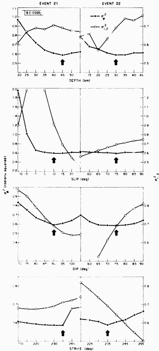
Fig. V-4. Results of fit to observed spectral ratios. \sigma^2_{1,2} is weighted sum of squares over frequency and station of observed log amplitude ratio minus theoretical log amplitude ratio. \sigma^2_{\phi} is similar weighted sum of squares of observed differential phases minus theoretical differential phase. For details, these quantities are given in Weibull and Aki. 8
