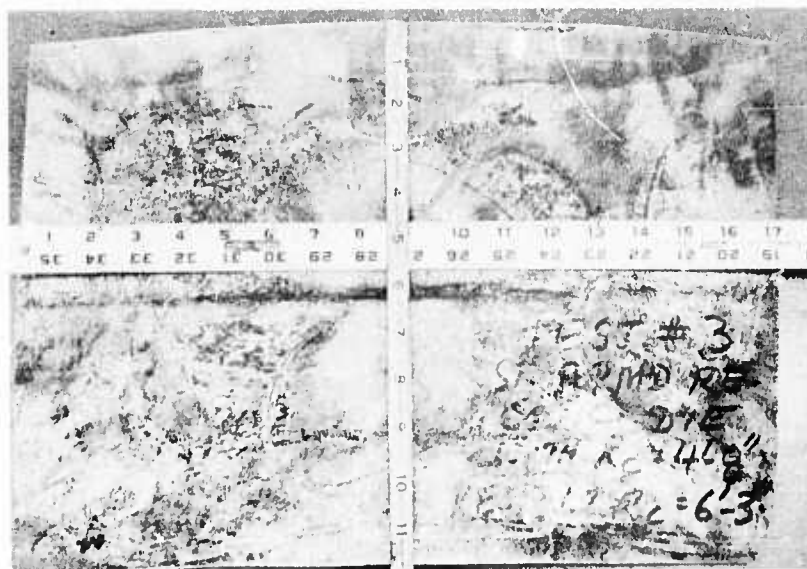
Figure 6. Gore Segment formed in Test 3. Outside view.
