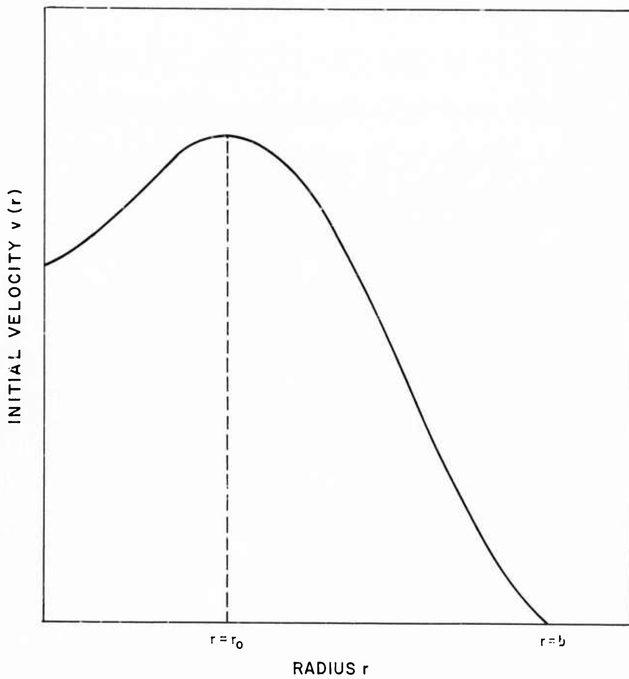
Figure 3. Diagram showing more general axi-symmetric initial velocity distribution.
