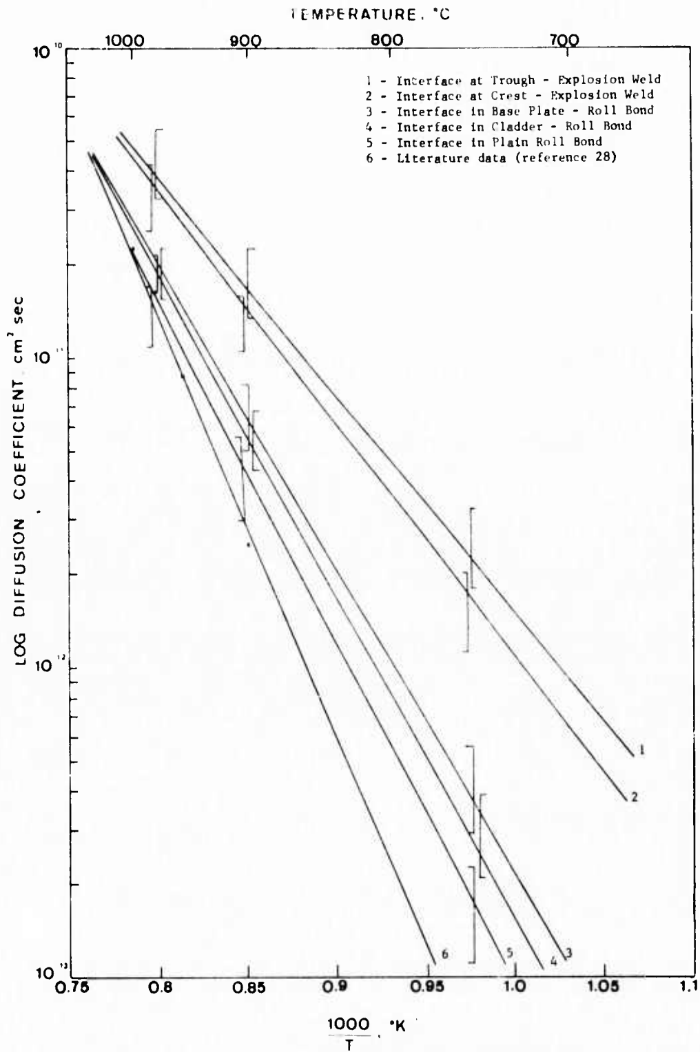
Figure 5. Diffusion coefficients for copper as a function of temperature at 50 atomic per cent copper in copper-nickel system. Copper-to-nickel specimen explosion welded with 1.24 g/cm. 2 loading.
