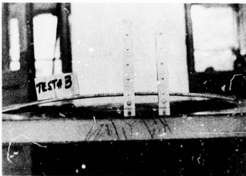
Figure 9. Gore Segment formed in Test 3. Side view.
