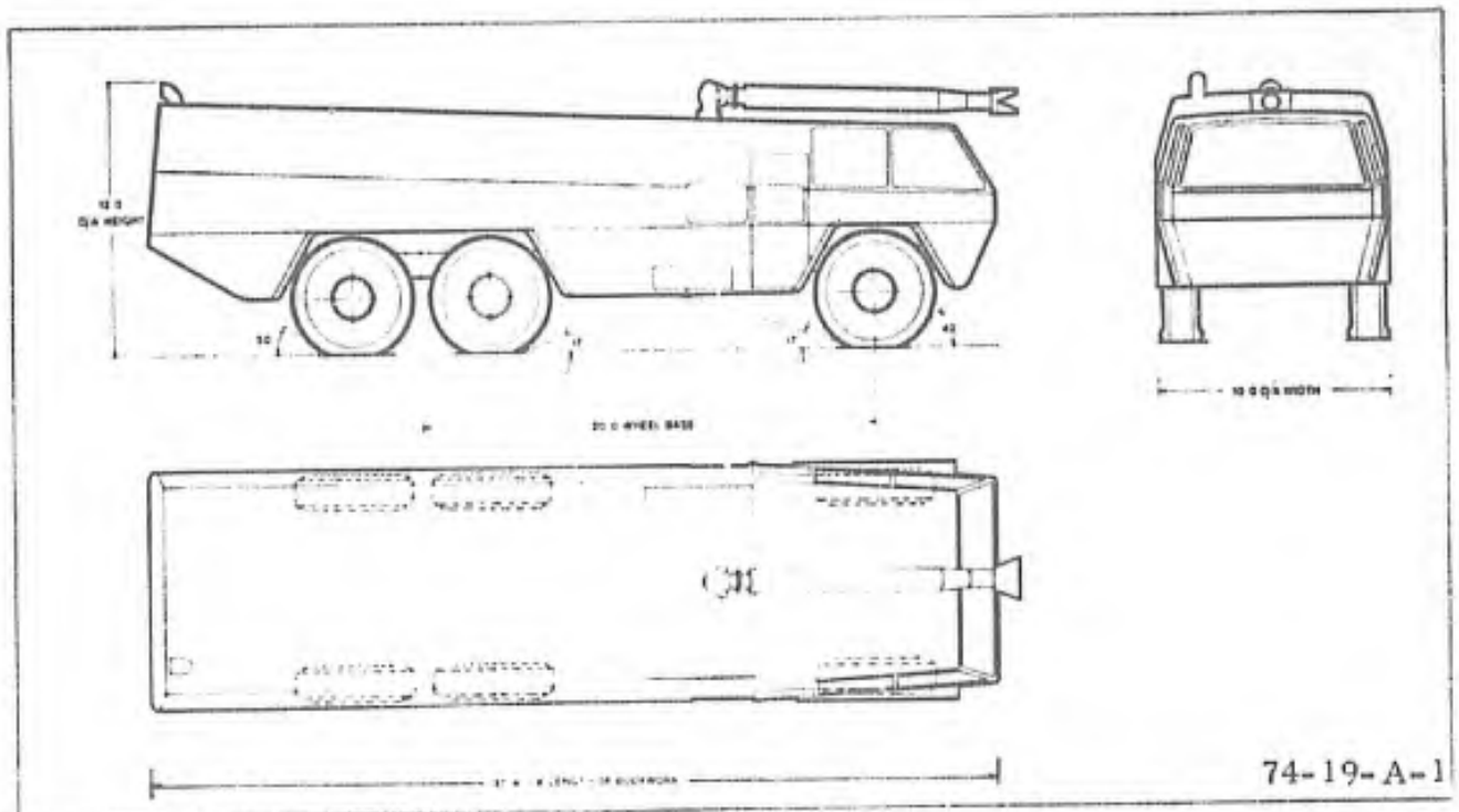
B. OVERALL DIMENSIONS OF THE FOAM TRUCK (FROM MANUFACTURER'S LITERATURE)
