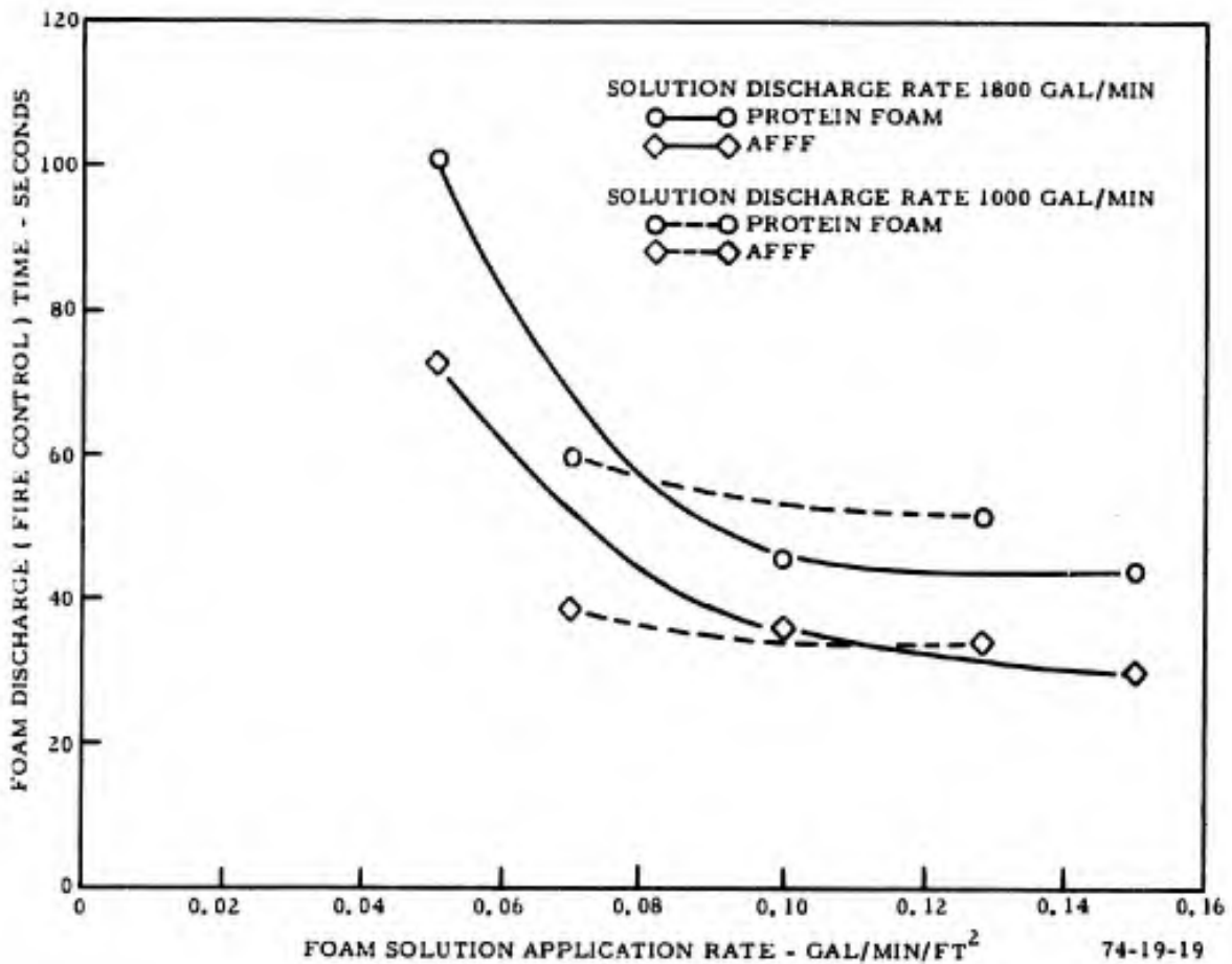
FIGURE 19. FOAM DISCHARGE (FIRE CONTROL) TIME AS A FUNCTION OF THE SOLUTION APPLICATION RATE USING PROTEIN FOAM AND AFFF
