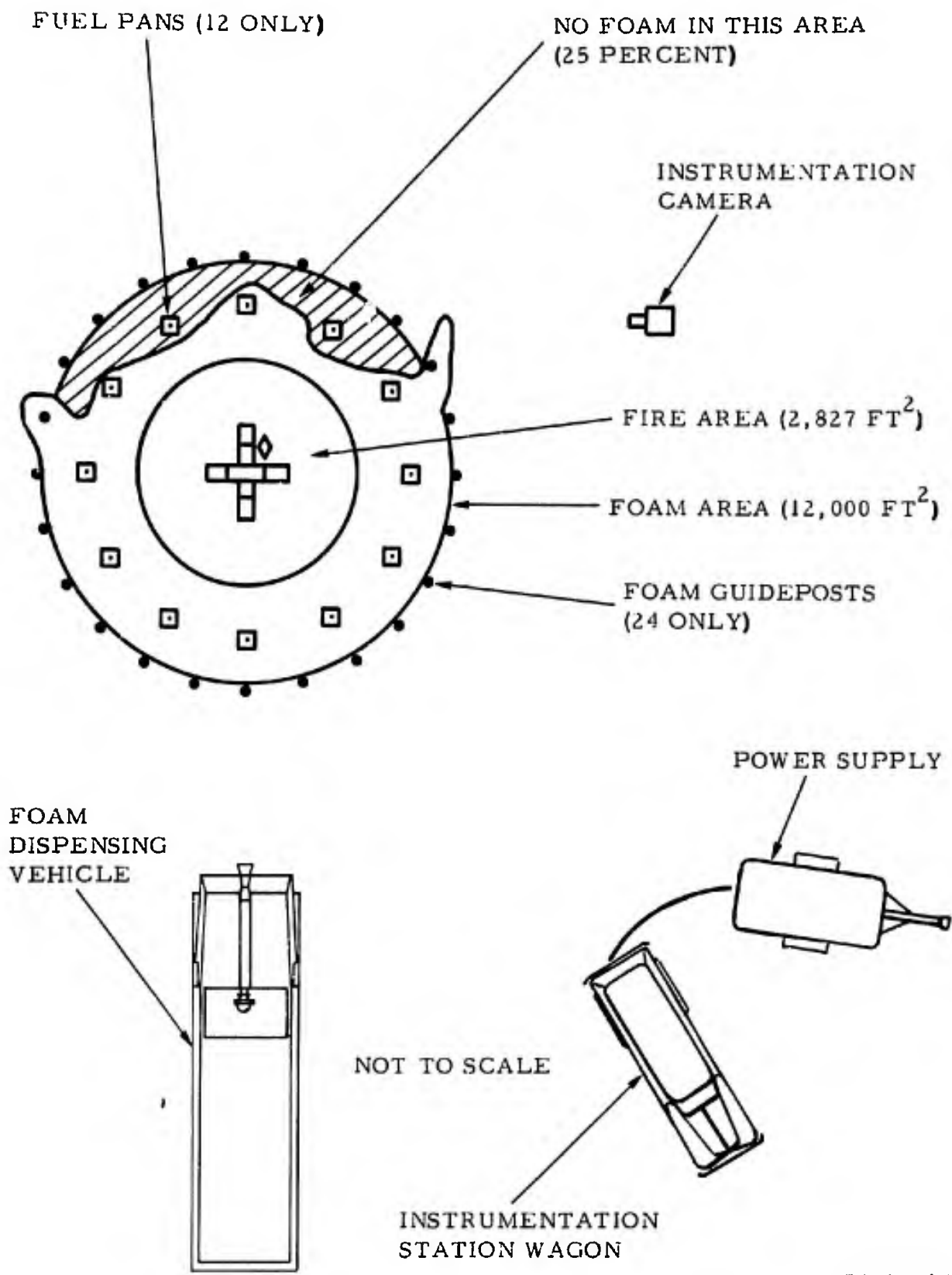
FIGURE 14. TEST 4 - CONFIGURATION OF THE FIRE TEST BED AND THE AREA OF AFFF COVERAGE
