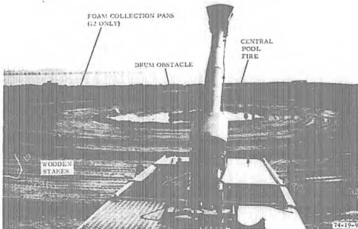
FIGURE 9. PICTORIAL VIEW OF THE FIRE TEST BED
