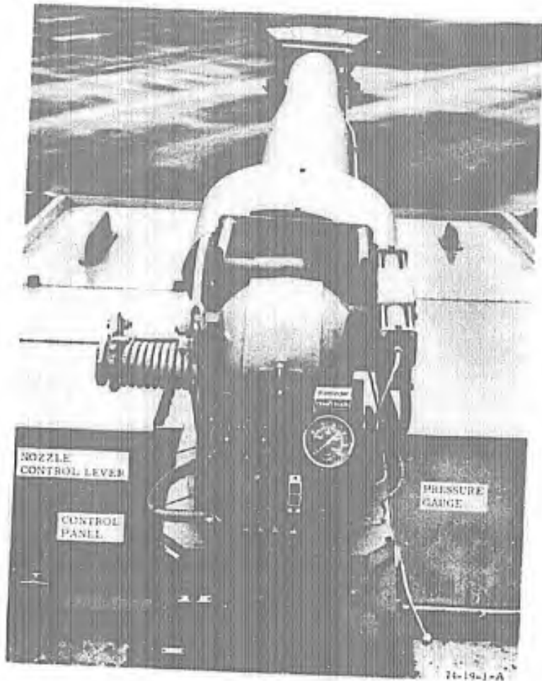
A. VIEW OF THE CONTROL PANEL FROM THE MONITOR PLATFORM
