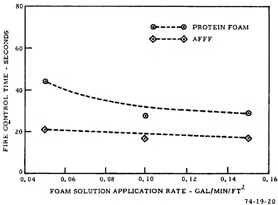
FIGURE 19. FOAM DISCHARGE (FIRE CONTROL) TIME AS A FUNCTION OF THE SOLUTION APPLICATION RATE USING PROTEIN FOAM AND AFFF
