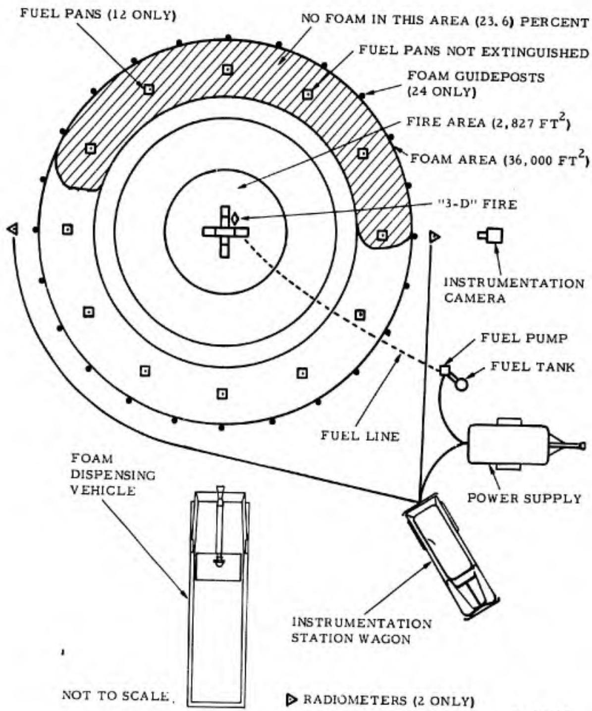
FIGURE 13. TEST 3 - CONFIGURATION OF THE FIRE TEST BED AND THE AREA OF PROTEIN FOAM COVERAGE
