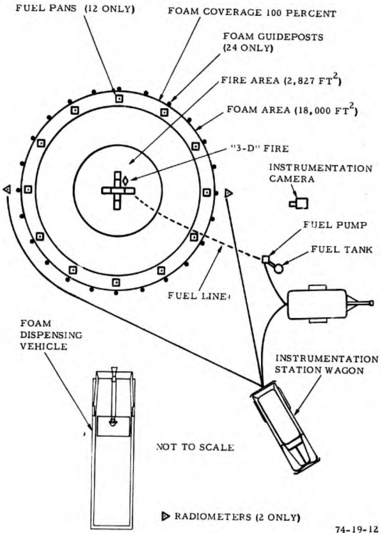
FIGURE 12. TEST 2 - CONFIGURATION OF THE FIRE TEST BED AND THE AREA OF PROTEIN FOAM COVERAGE
