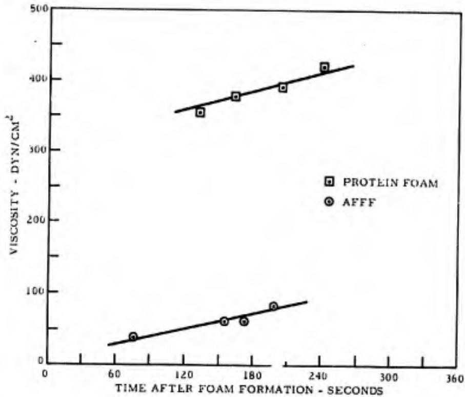
FIGURE 7. VISCOSITY OF PROTEIN FOAM AND AFFF AS A FUNCTION OF THE TIME AFTER FORMATION
