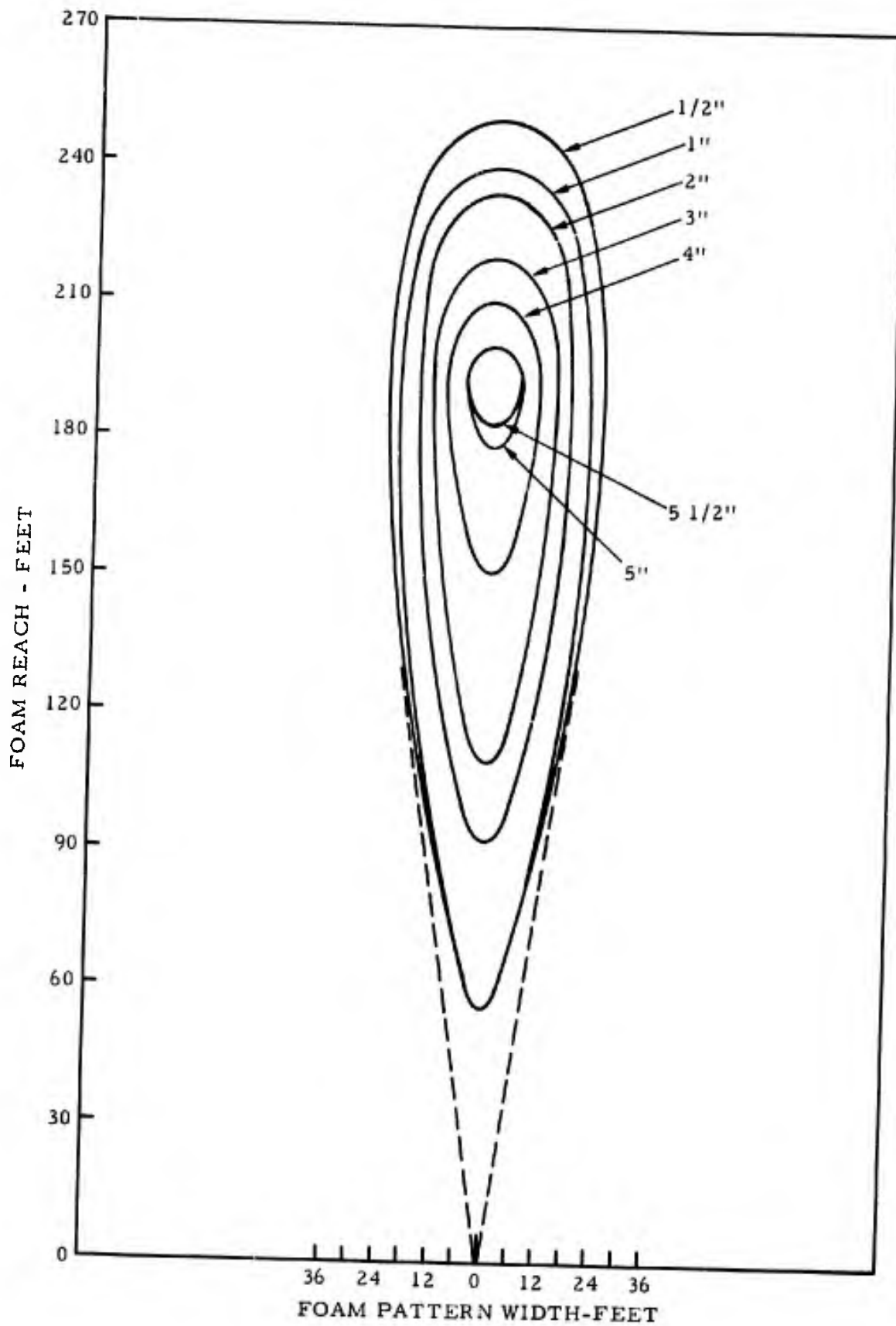
FIGURE 4. PROTEIN FOAM DEPTH CONTOUR OBTAINED AT A SOLUTION RATE OF 1,800 GAL/MIN USING THE STRAIGHT-STREAM DISCHARGE
