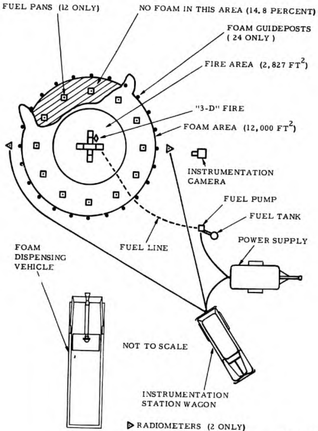
FIGURE 11. TEST 1 - CONFIGURATION OF THE FIRE TEST BED AND THE AREA OF PROTEIN FOAM COVERAGE
