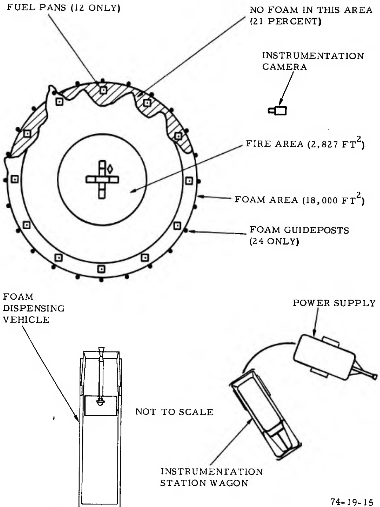
FIGURE 15. TEST 5 - CONFIGURATION OF THE FIRE TEST BED AND THE AREA OF AFFF COVERAGE
