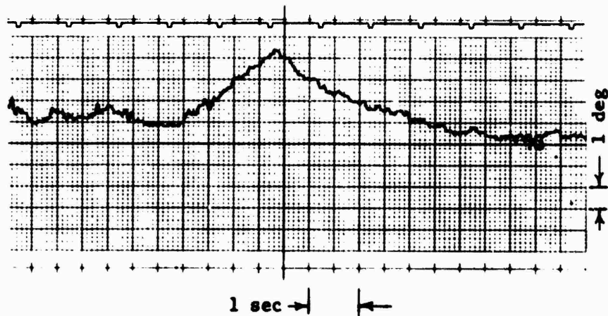
Free Roll Oscillation, V = 25.5 Knots
