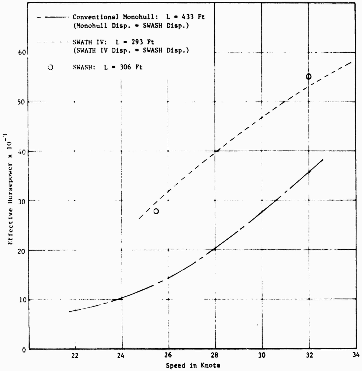
Figure 23- Effective Horsepower for SWASH, SWATH IV and a Conventional Monohull
