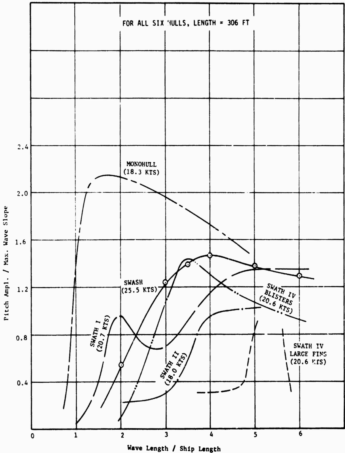
Figure 6 - Comparison of Pitch Transfer Functions Obtained in Head Regular Waves for SWASH, SWATH, and a Conventional Monohull; SWASH Speed = 25.5 Knots
