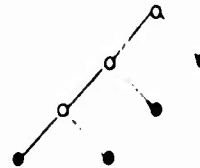
Frontier of fathomed nodes for "collapsed" tree (denoted by \bullet )
