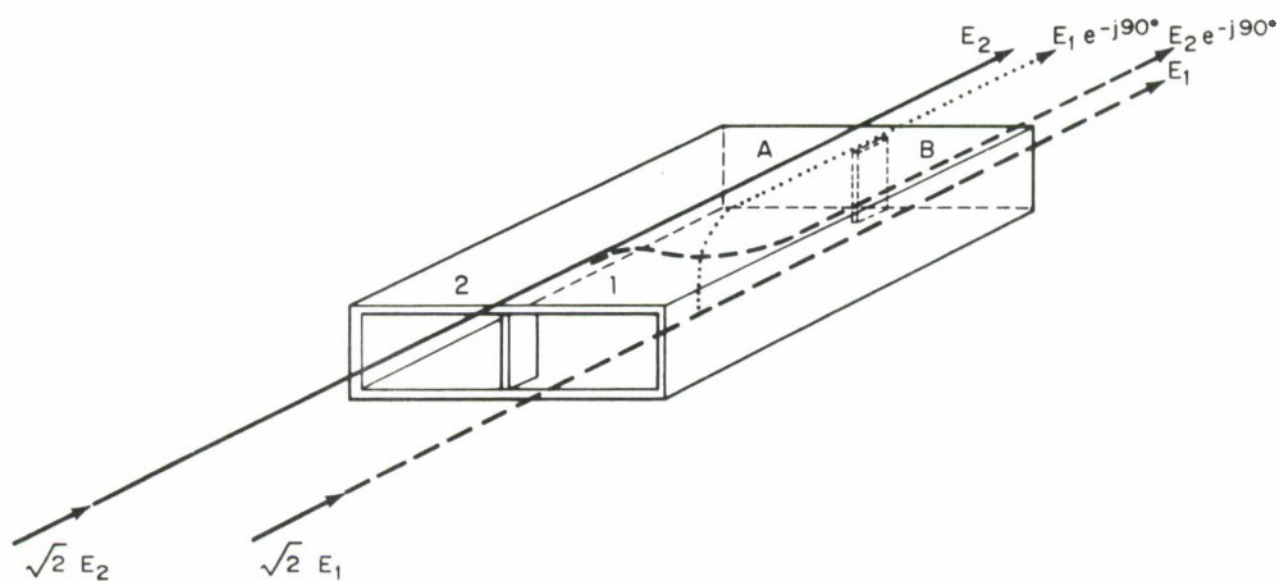
Fig. 3. 3 dB hybrid coupler.
