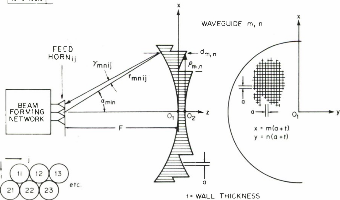
Fig. 8. Lens and feed geometry.
