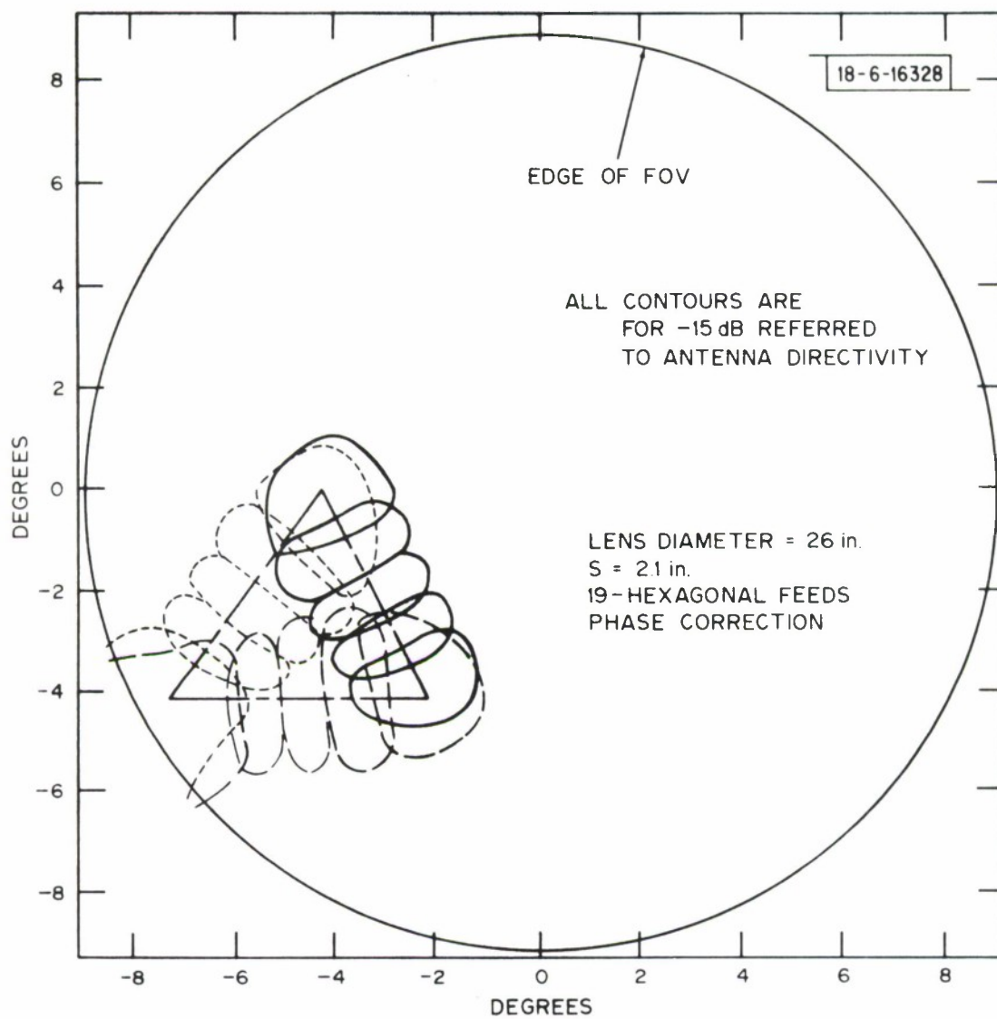
Fig. 19. Composite radiation patterns for null steering.
