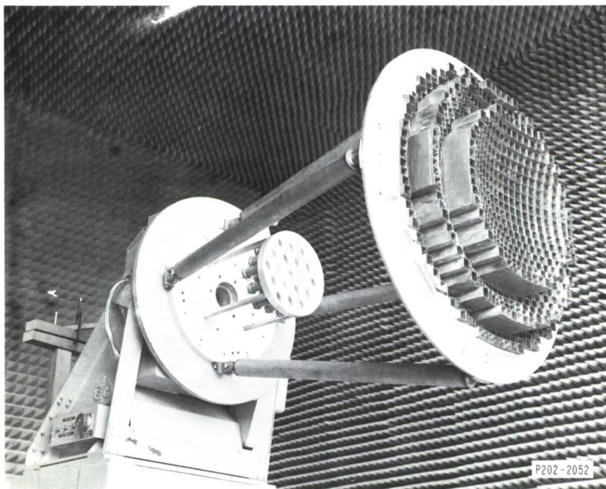
Fig. 1. LES-7 multiple beam lens antenna.
