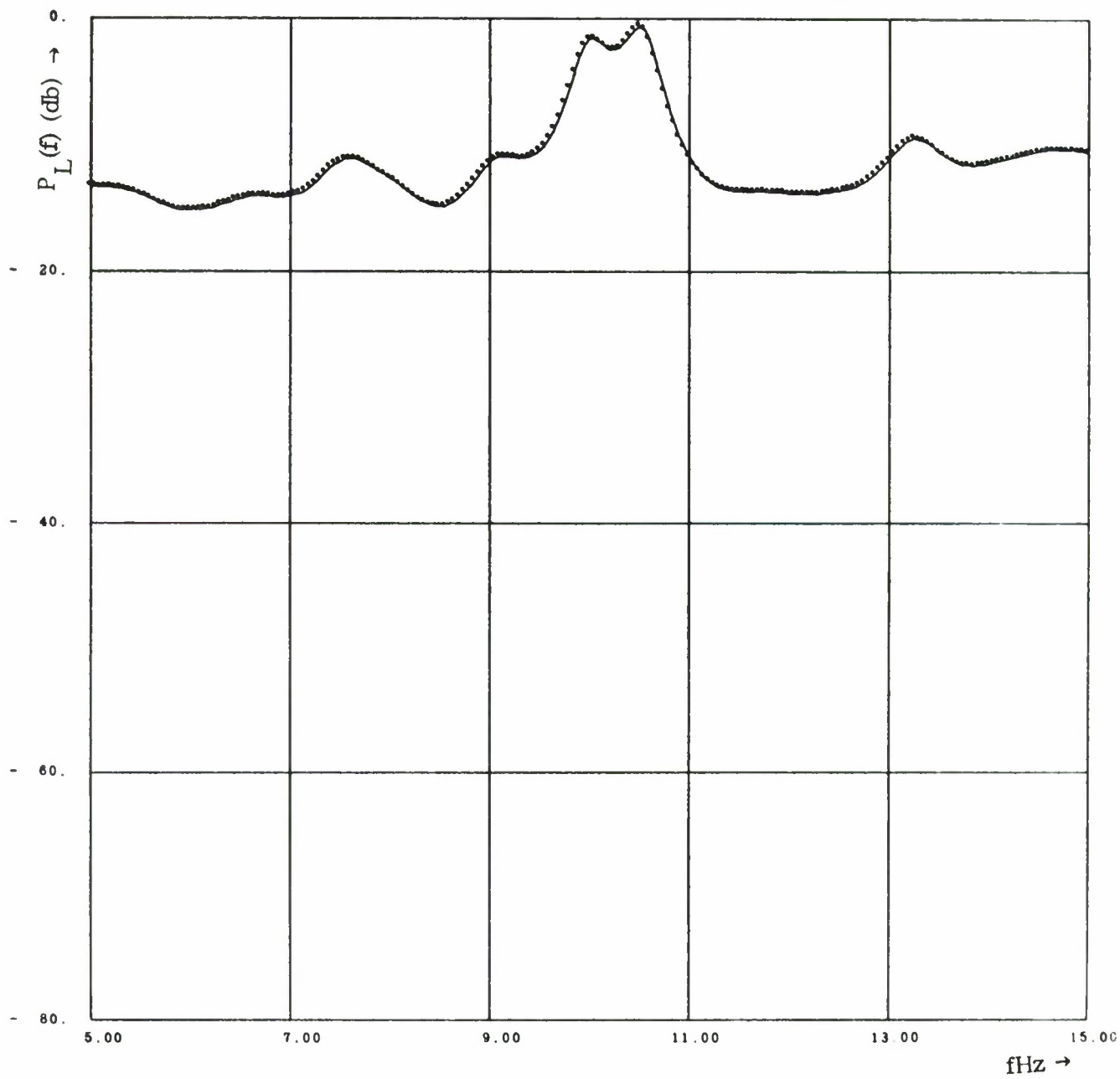
Fig. 5.29 - Indirect, \rho = .3 .
