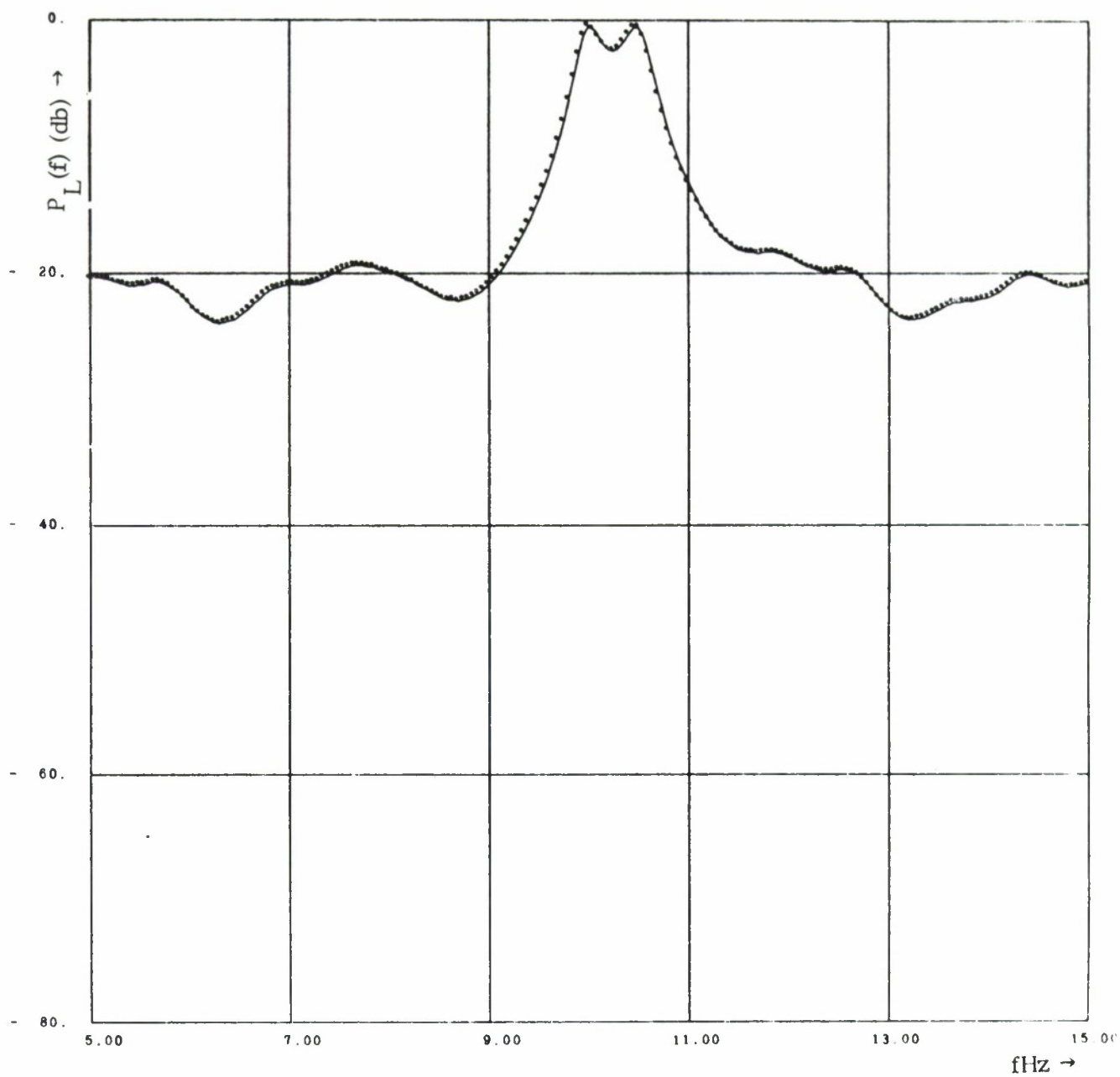
Fig. 5.5 - Indirect, \rho = .3 .
