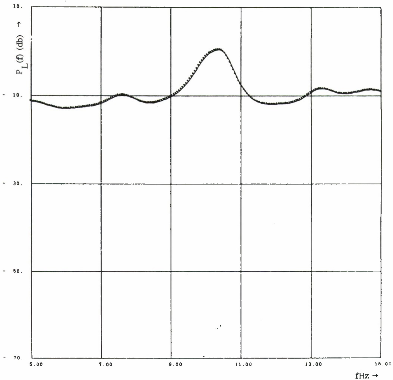
Fig. 5.27 - Indirect, \rho = .2 .
