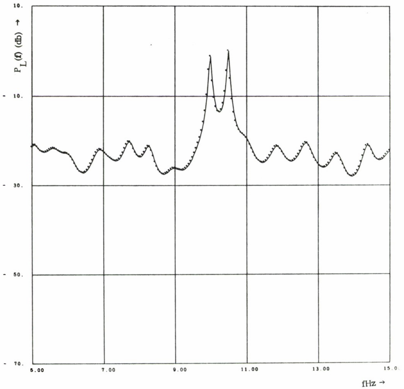
Fig. 5.8 - Direct, \rho = .4 .
