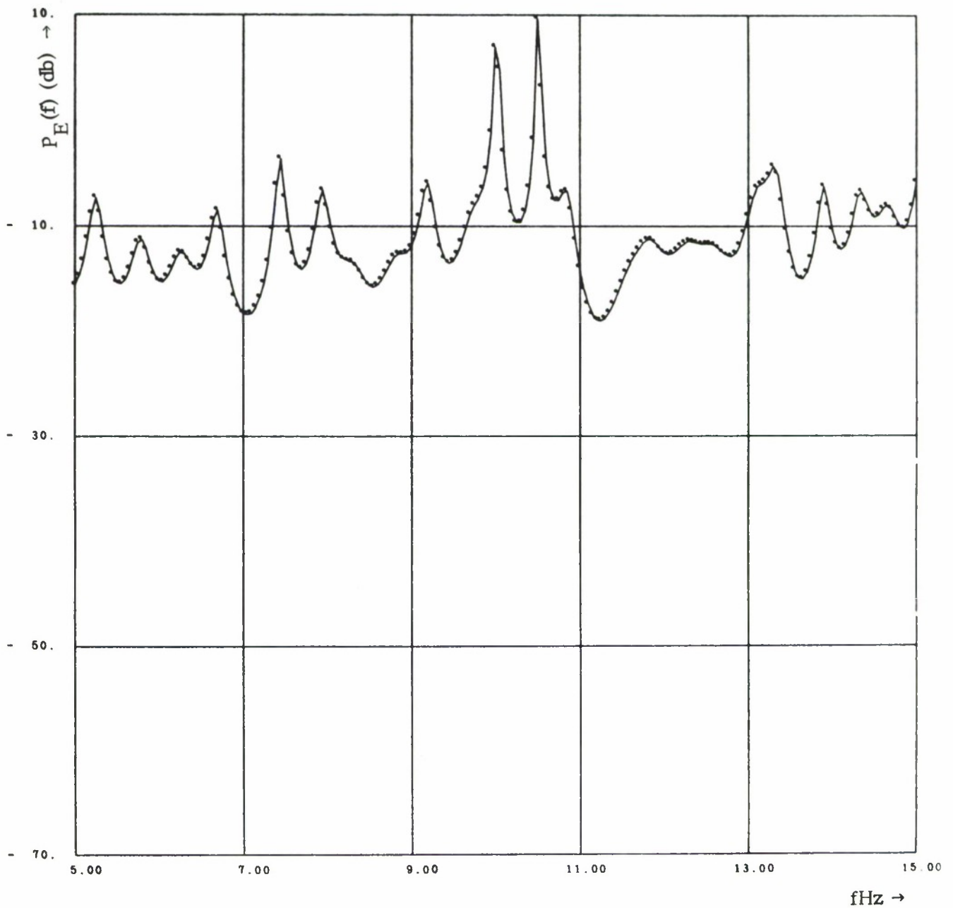
Fig. 5.48 - Direct-Hanning, \rho = .5 .
