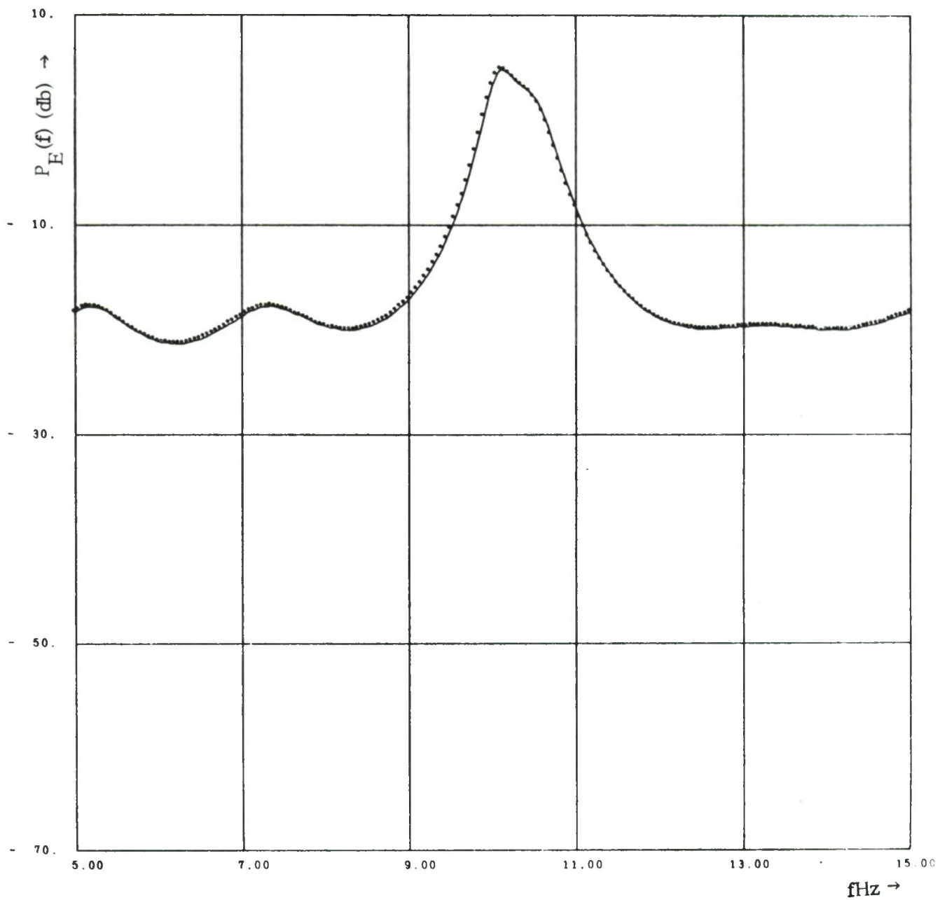
Fig. 5.13 - Indirect, \rho = .1 .
