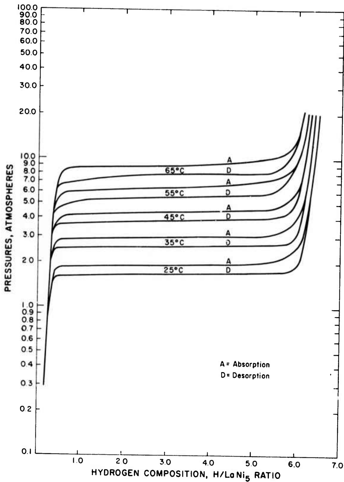
Figure 15. Family of Isotherms in Absorption and Desorption of the \text{LaNi}_5 -H System from 25 to 65°C.
