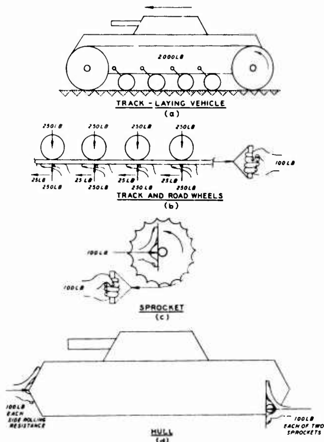
Fig. A3. Track-laying mode
