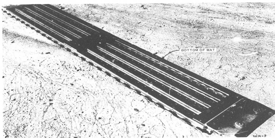
Fig. 5. M9M1 landing mat
