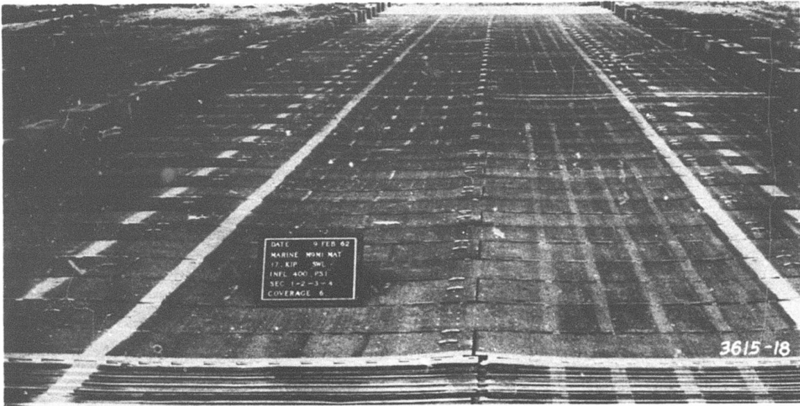
Photograph 3. Test section with staggered end joints after 6 coverages
