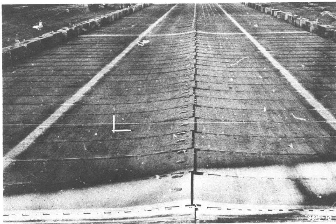
Photograph 2. Test section with end joints in straight line after 6 coverages. Note deformation of planks
