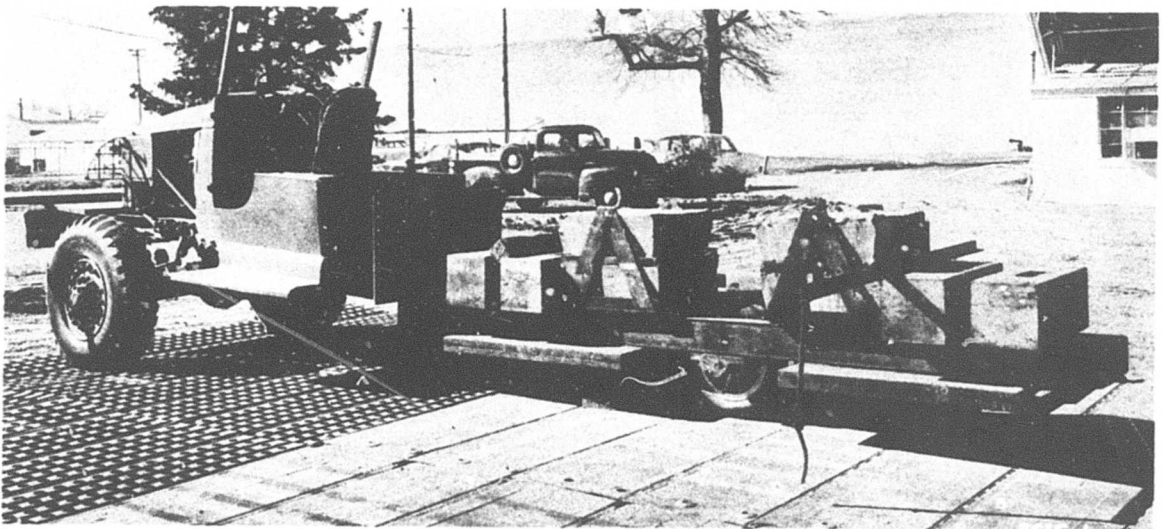
Fig. 6. Single-wheel test load cart
