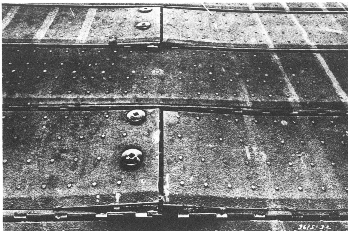
Photograph 10. Close-up of item 2 after 128 coverages
