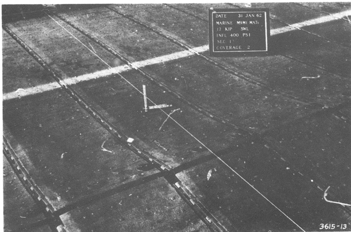
Photograph 1. Item 1 after 2 coverages had caused end joints to arch up
