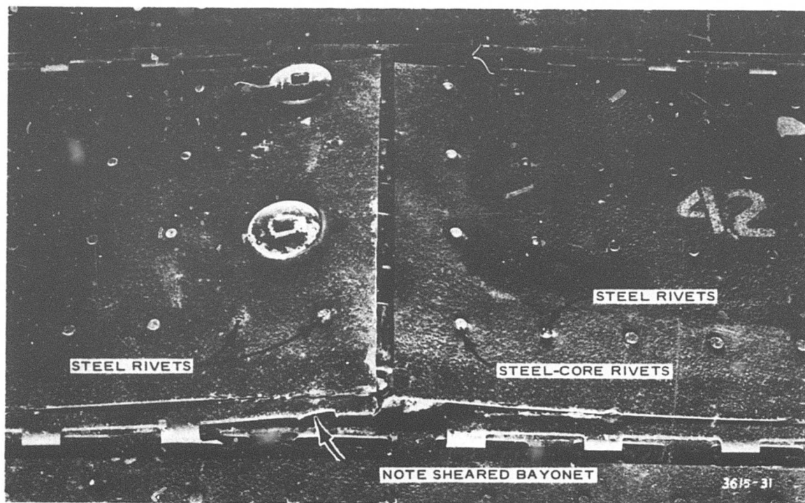
Fig. 9. Condition of steel rivets in plank after 78 coverages. Note sheared bayonet and end curl
