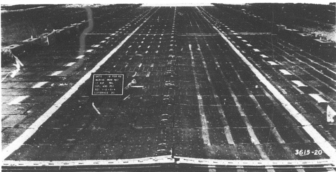
Photograph 4. Test section with staggered end joints after 20 coverages
