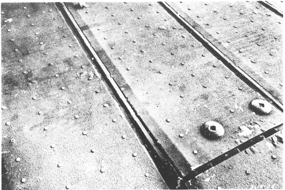
Photograph 14. Close-up of item 4 after 128 coverages
