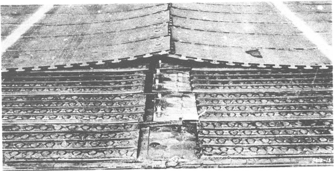
Fig. 8. Sheared end plates after six coverages
