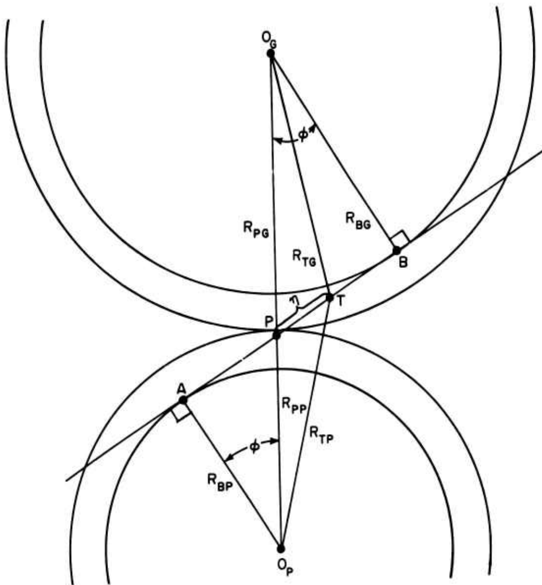
Figure 100. Geometry Associated With Gear Pair.
