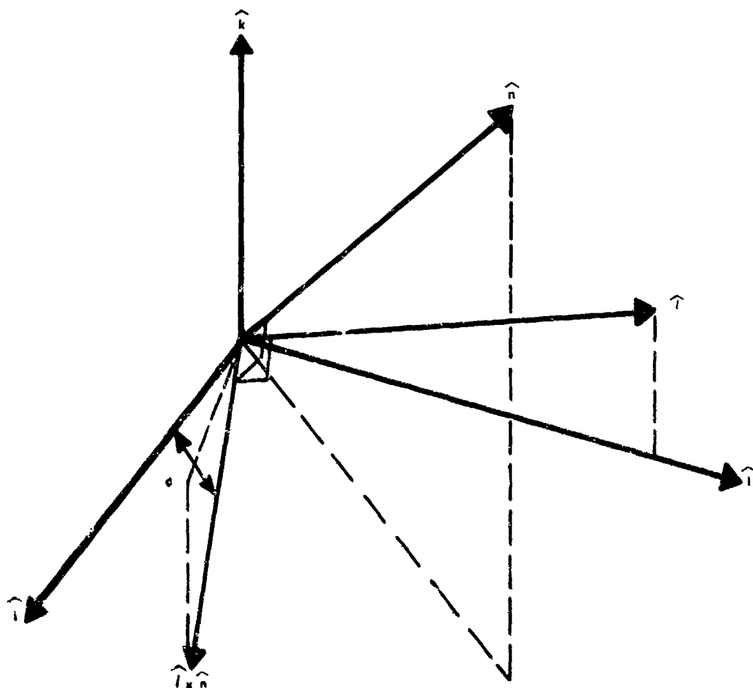
Figure 4. Relation Between the Local and Macrosurface Plane of Incidence. The vectors \hat{i} and \hat{k} lie in the macrosurface plane of incidence, and \hat{i} and \hat{n} lie in the local plane of incidence. The angle between these planes is equal to \phi (the angle between their normals).
