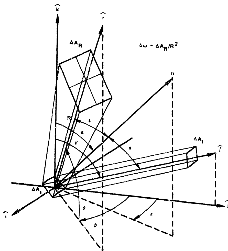
Figure 1. Reflection From a Curved Microarea of the Rough-Surface Air/Material Interface. A small, optically smooth, slightly curved area \Delta A_R with a normal \hat{n} intercepts the light from an area \Delta A_I of the incident beam and diverges it into \Delta\omega steradians in a direction \hat{r} such that \hat{r} \times \hat{n} = \hat{n} \times \hat{l} .
