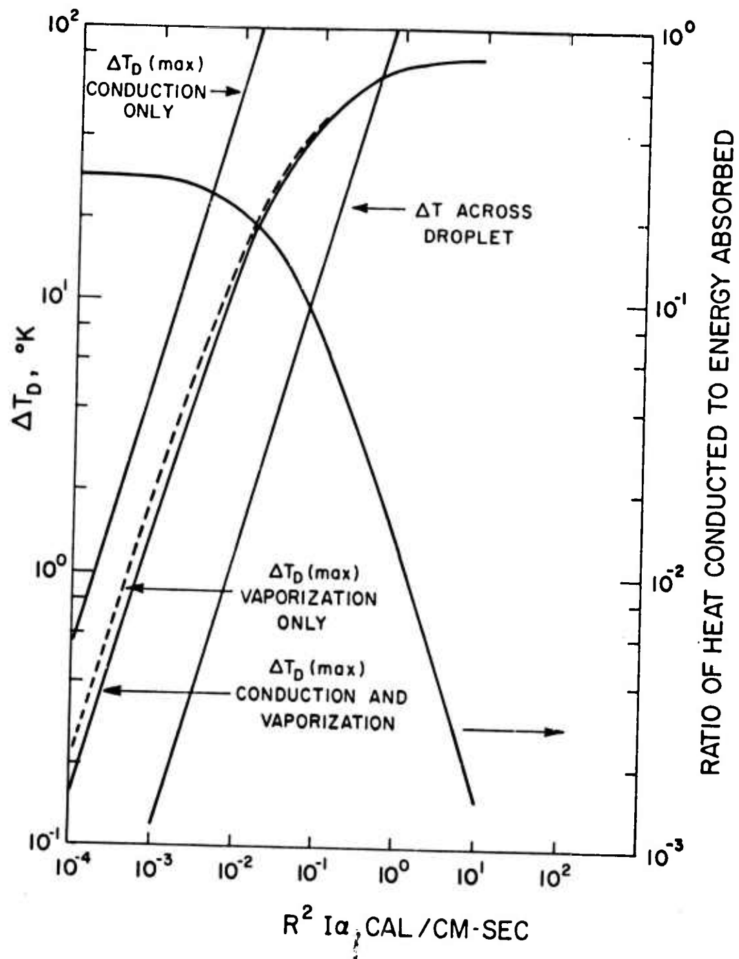
Fig. 4 Maximum Increase in Droplet Temperature vs. R^2 I \alpha . Also shown is the fraction of absorbed energy lost to heat conduction and the predicted variation in temperature across the droplet.
